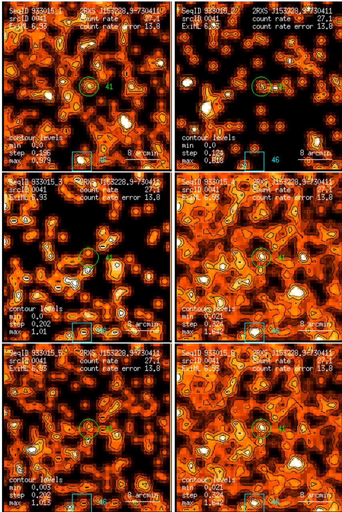
Figure 41: RASS 933015: detection 0041: band rate images, Gaussian filter: (1) PSPC channels 11 – 41, (2) 52 – 90, (3) 91 – 201, (4) 11 – 235, (5) 52 – 201, (6) 11 – 201. Broad band rates in counts/ks. Band rate contour levels in counts/ks/arcmin 2 .
