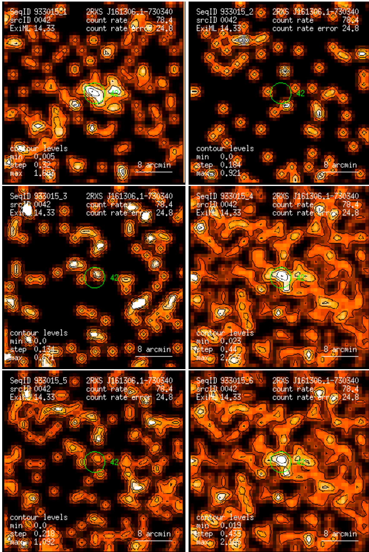
Figure 42: RASS 933015: detection 0042: band rate images, Gaussian filter: (1) PSPC channels 11 – 41, (2) 52 – 90, (3) 91 – 201, (4) 11 – 235, (5) 52 – 201, (6) 11 – 201. Broad band rates in counts/ks. Band rate contour levels in counts/ks/arcmin 2 .
