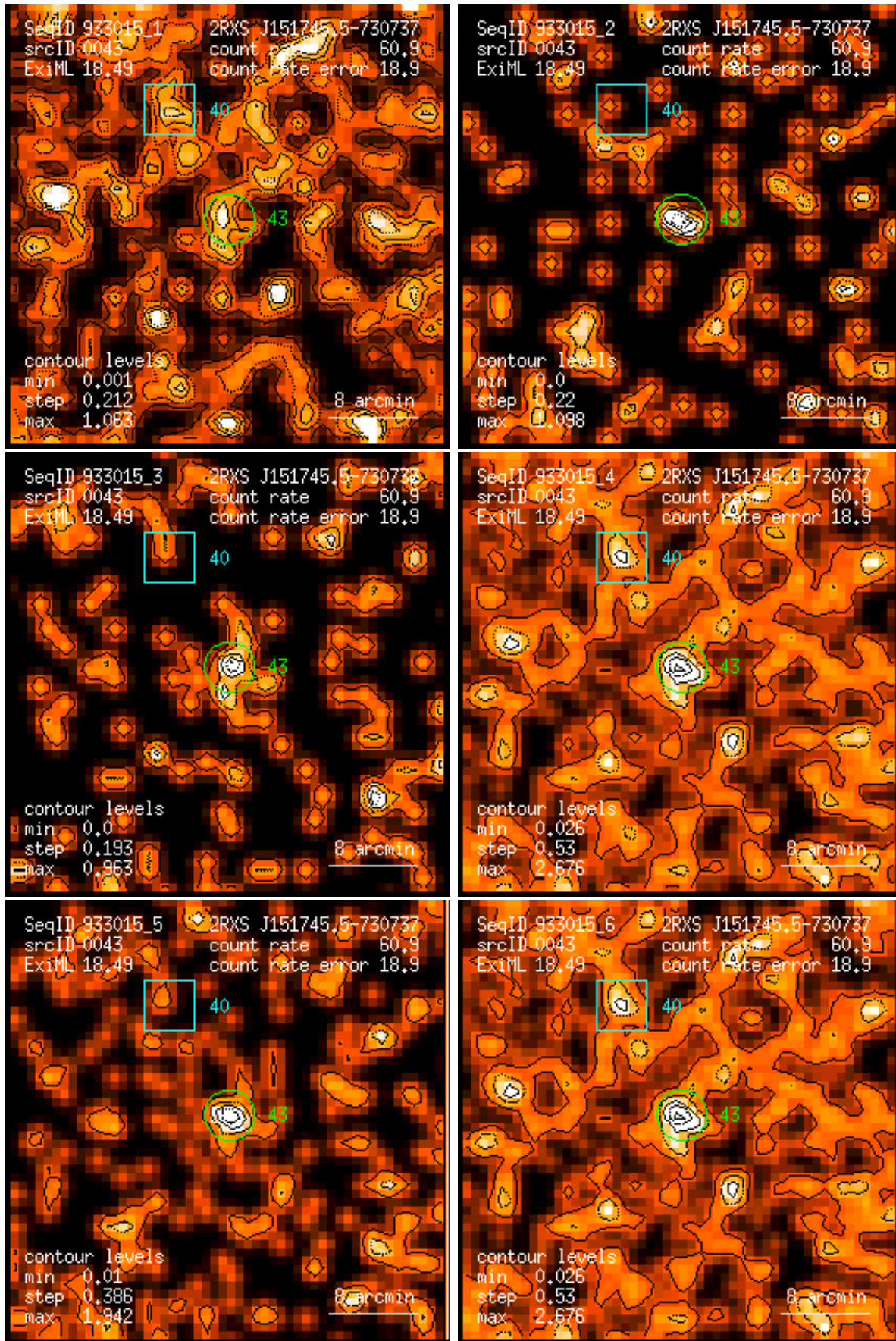
Figure 43: RASS 933015: detection 0043: band rate images, Gaussian filter: (1) PSPC channels 11 – 41, (2) 52 – 90, (3) 91 – 201, (4) 11 – 235, (5) 52 – 201, (6) 11 – 201. Broad band rates in counts/ks. Band rate contour levels in counts/ks/arcmin 2 .
