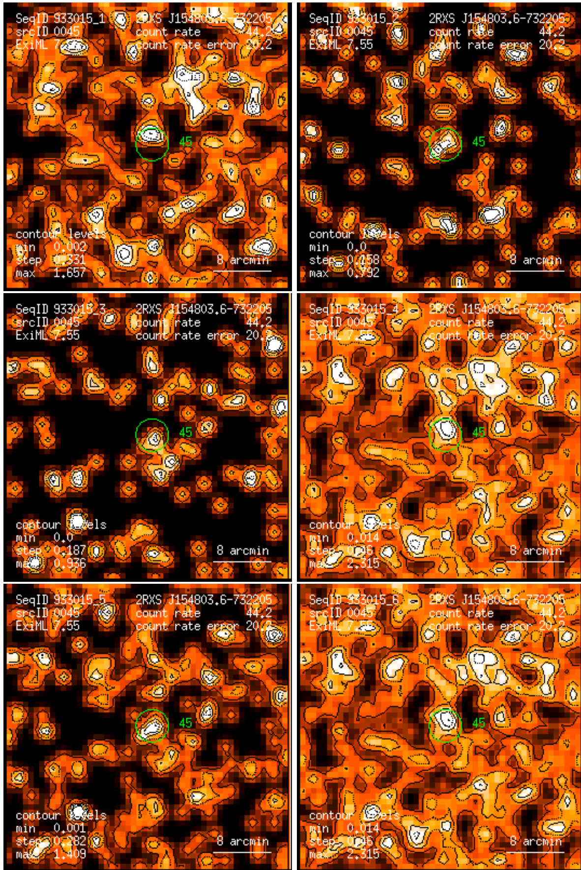
Figure 45: RASS 933015: detection 0045: band rate images, Gaussian filter: (1) PSPC channels 11 – 41, (2) 52 – 90, (3) 91 – 201, (4) 11 – 235, (5) 52 – 201, (6) 11 – 201. Broad band rates in counts/ks. Band rate contour levels in counts/ks/arcmin 2 .
