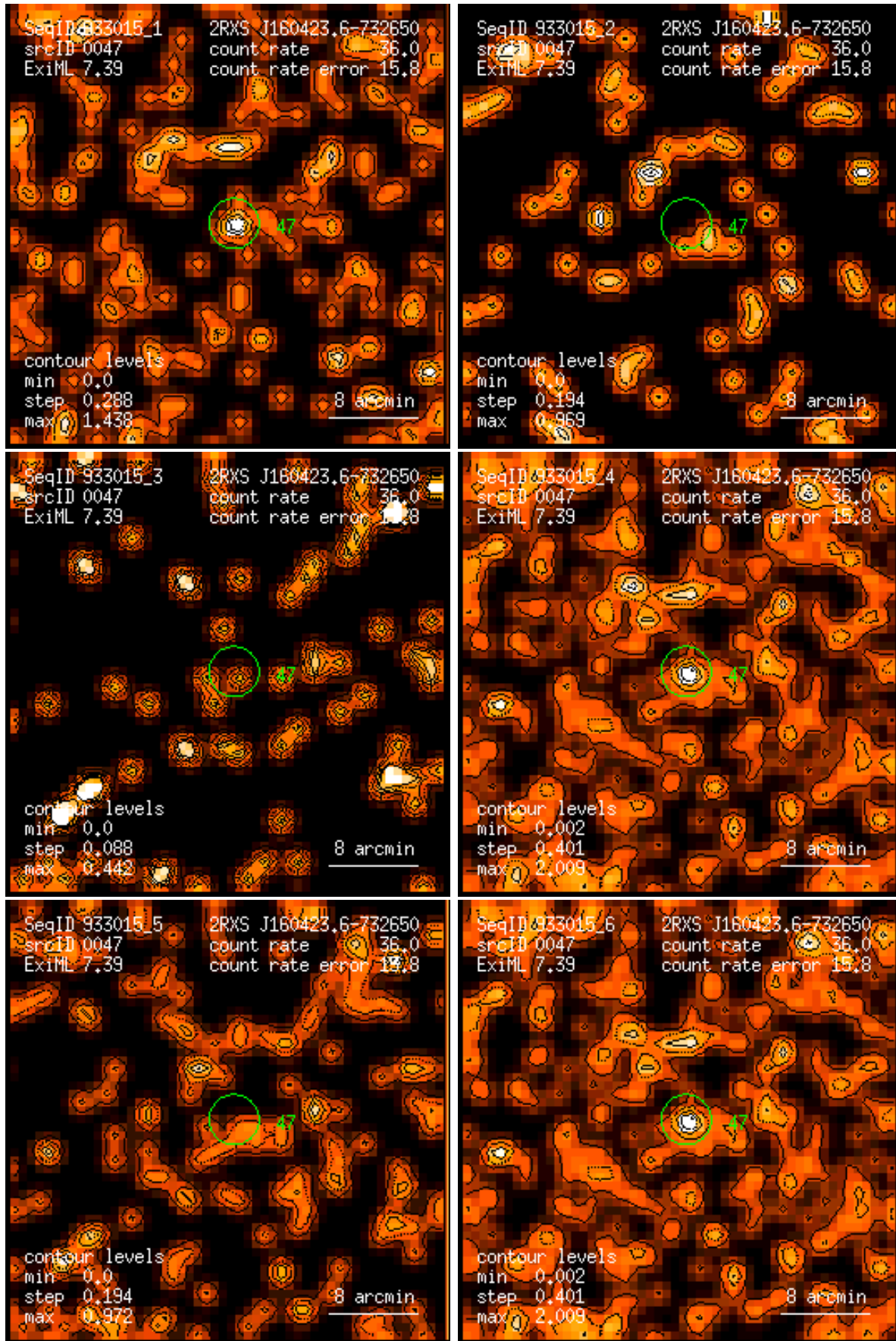
Figure 47: RASS 933015: detection 0047: band rate images, Gaussian filter: (1) PSPC channels 11 – 41, (2) 52 – 90, (3) 91 – 201, (4) 11 – 235, (5) 52 – 201, (6) 11 – 201. Broad band rates in counts/ks. Band rate contour levels in counts/ks/arcmin 2 .
