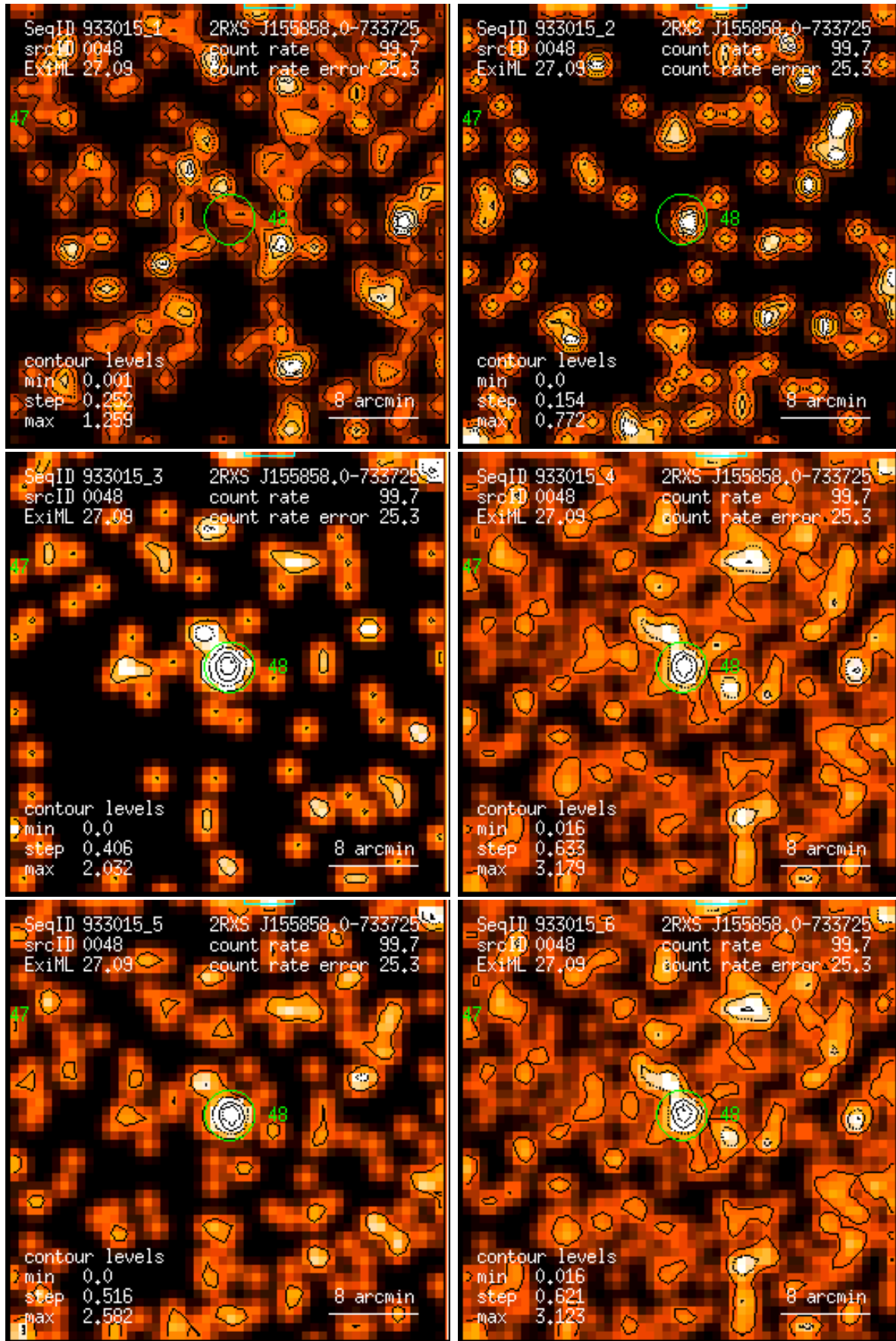
Figure 48: RASS 933015: detection 0048: band rate images, Gaussian filter: (1) PSPC channels 11 – 41, (2) 52 – 90, (3) 91 – 201, (4) 11 – 235, (5) 52 – 201, (6) 11 – 201. Broad band rates in counts/ks. Band rate contour levels in counts/ks/arcmin 2 .
