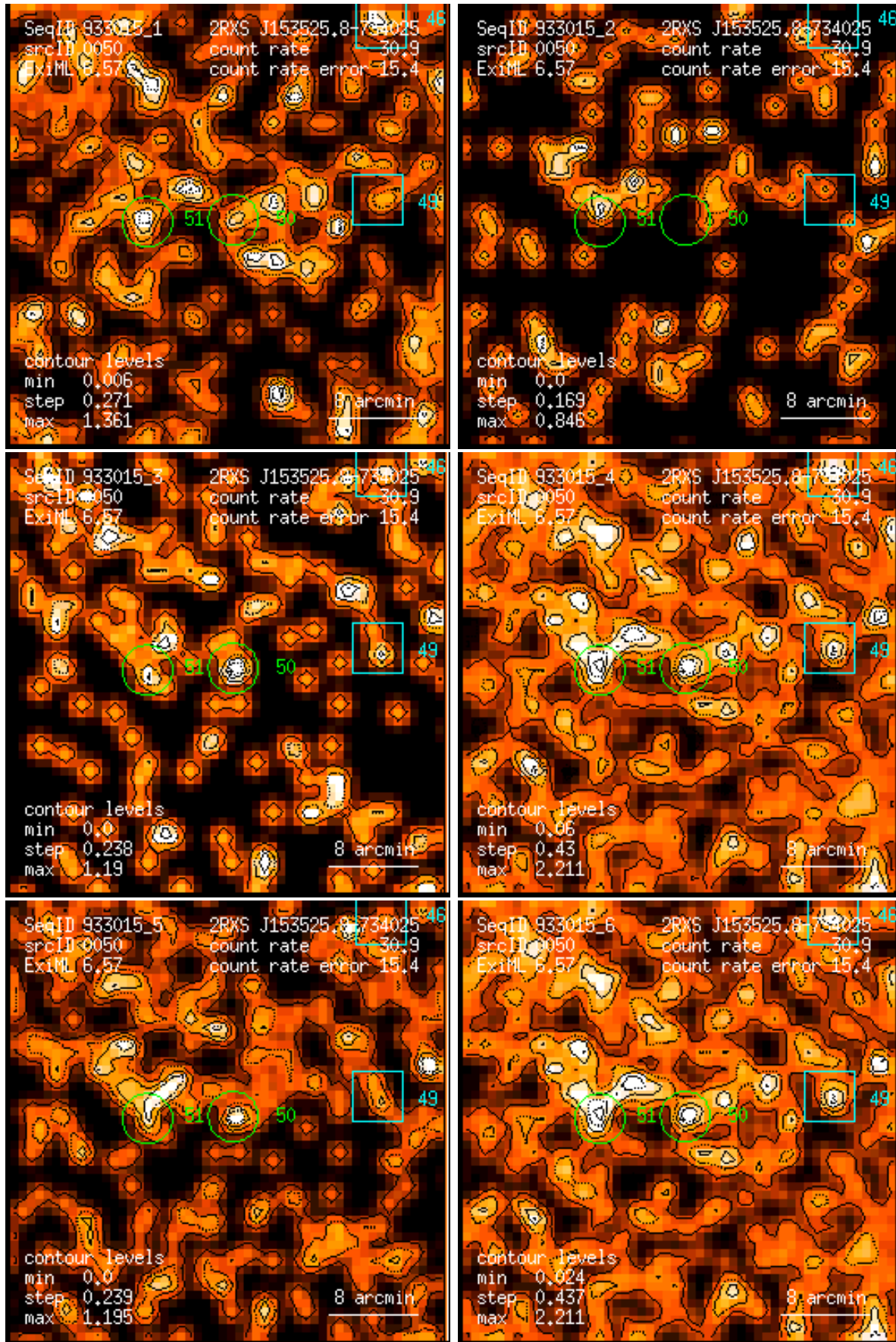
Figure 50: RASS 933015: detection 0050: band rate images, Gaussian filter: (1) PSPC channels 11 – 41, (2) 52 – 90, (3) 91 – 201, (4) 11 – 235, (5) 52 – 201, (6) 11 – 201. Broad band rates in counts/ks. Band rate contour levels in counts/ks/arcmin 2 .
