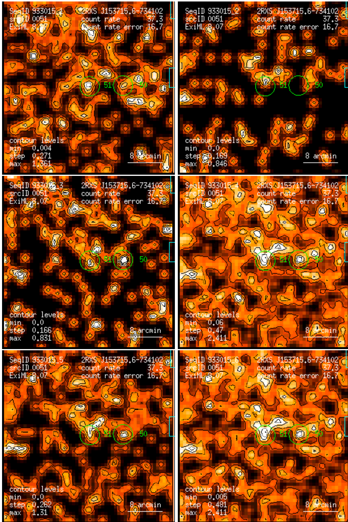
Figure 51: RASS 933015: detection 0051: band rate images, Gaussian filter: (1) PSPC channels 11 – 41, (2) 52 – 90, (3) 91 – 201, (4) 11 – 235, (5) 52 – 201, (6) 11 – 201. Broad band rates in counts/ks. Band rate contour levels in counts/ks/arcmin 2 .
