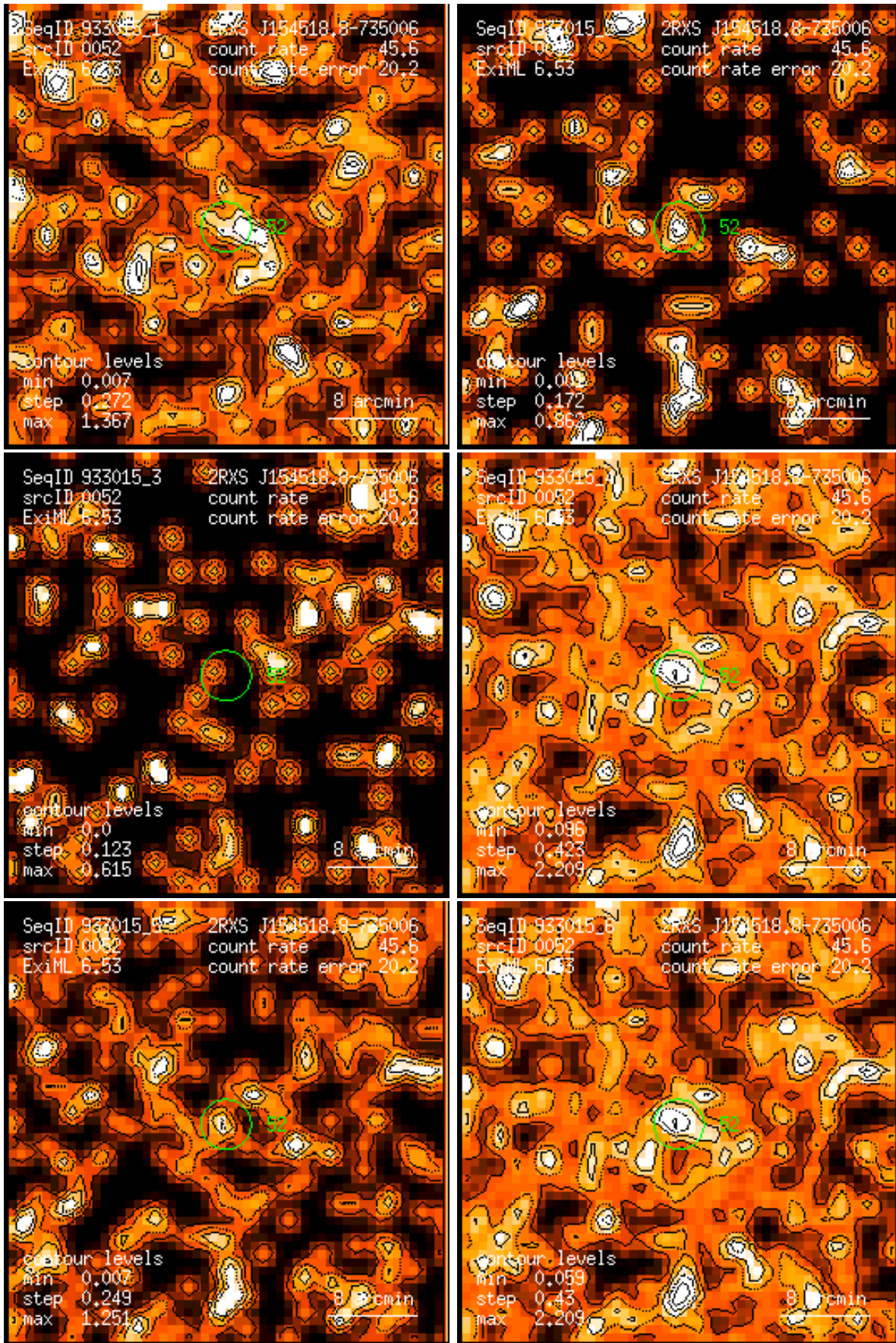
Figure 52: RASS 933015: detection 0052: band rate images, Gaussian filter: (1) PSPC channels 11 – 41, (2) 52 – 90, (3) 91 – 201, (4) 11 – 235, (5) 52 – 201, (6) 11 – 201. Broad band rates in counts/ks. Band rate contour levels in counts/ks/arcmin 2 .
