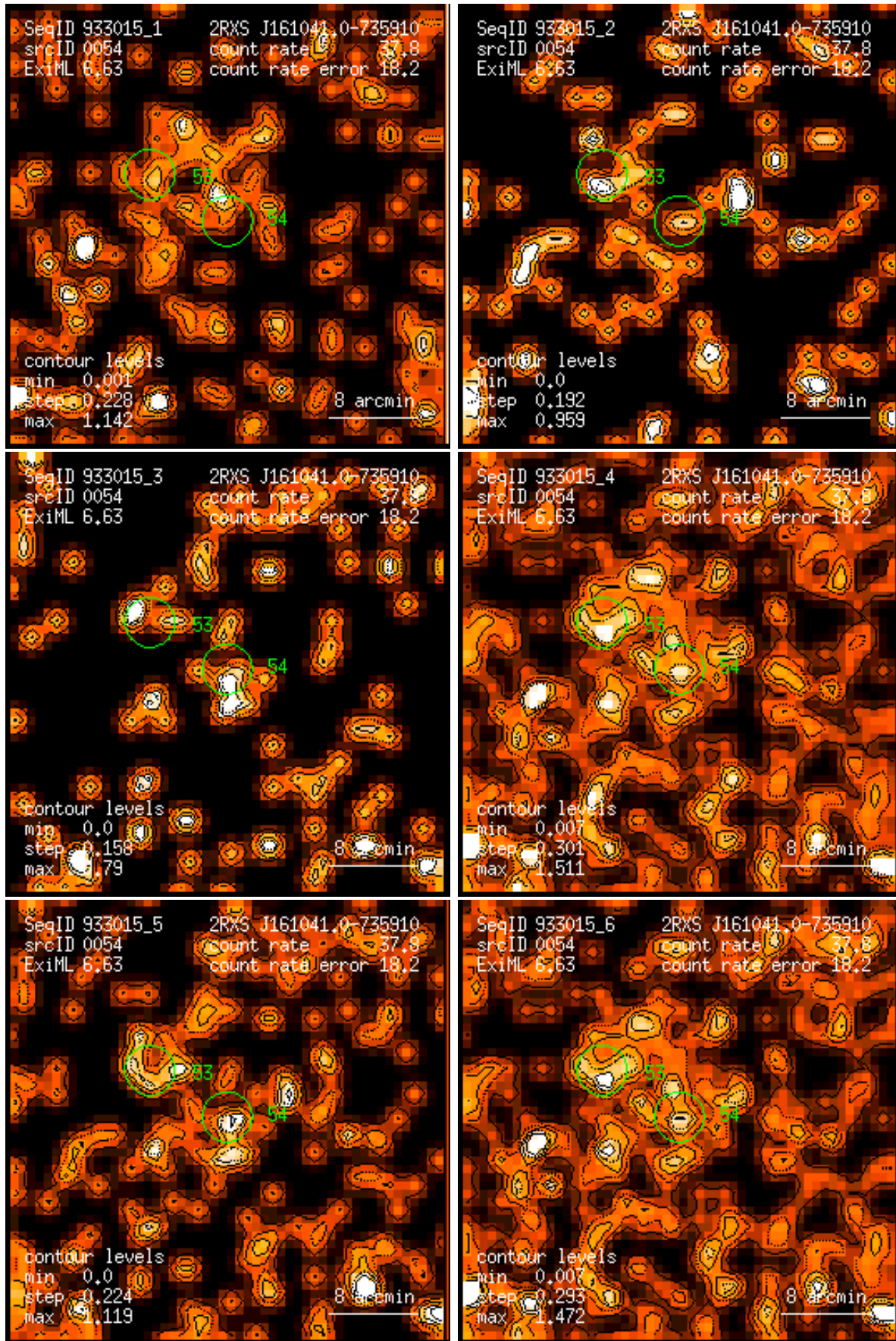
Figure 54: RASS 933015: detection 0054: band rate images, Gaussian filter: (1) PSPC channels 11 – 41, (2) 52 – 90, (3) 91 – 201, (4) 11 – 235, (5) 52 – 201, (6) 11 – 201. Broad band rates in counts/ks. Band rate contour levels in counts/ks/arcmin 2 .
