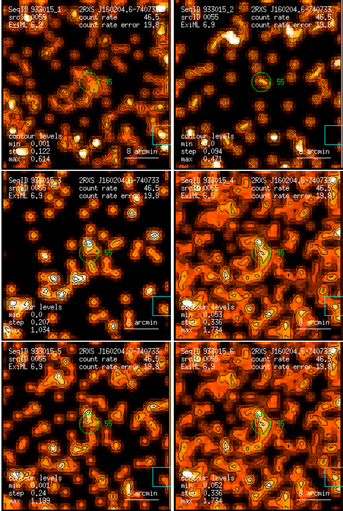
Figure 55: RASS 933015: detection 0055: band rate images, Gaussian filter: (1) PSPC channels 11 – 41, (2) 52 – 90, (3) 91 – 201, (4) 11 – 235, (5) 52 – 201, (6) 11 – 201. Broad band rates in counts/ks. Band rate contour levels in counts/ks/arcmin 2 .
