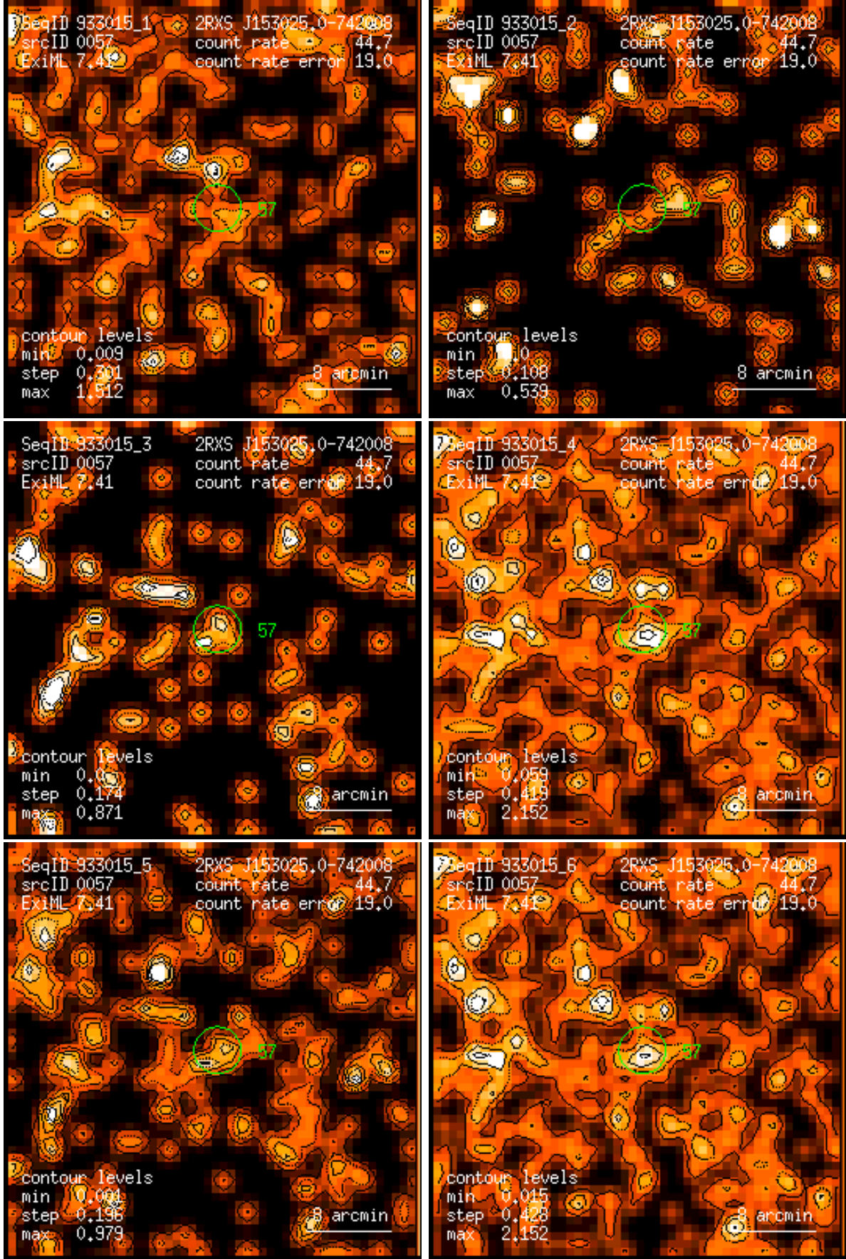
Figure 57: RASS 933015: detection 0057: band rate images, Gaussian filter: (1) PSPC channels 11 – 41, (2) 52 – 90, (3) 91 – 201, (4) 11 – 235, (5) 52 – 201, (6) 11 – 201. Broad band rates in counts/ks. Band rate contour levels in counts/ks/arcmin 2 .
