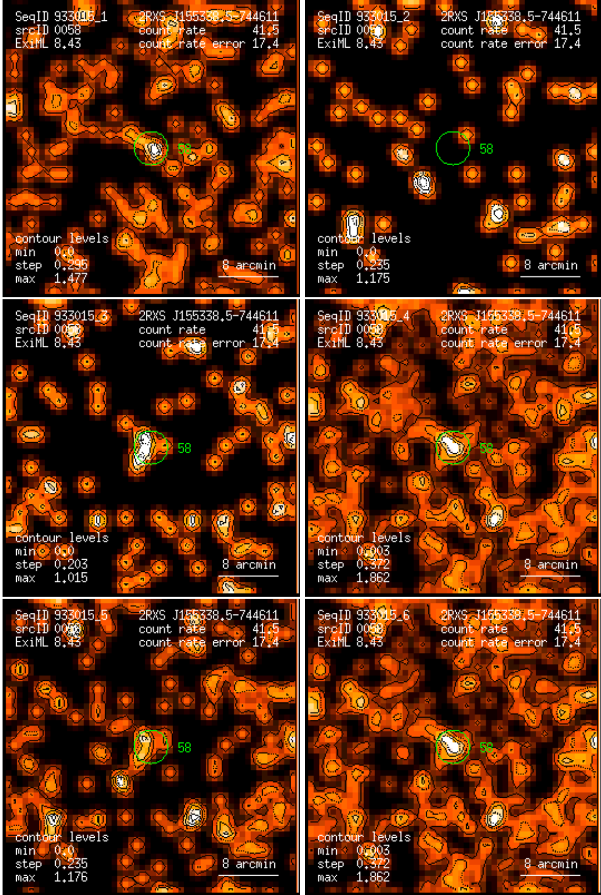
Figure 58: RASS 933015: detection 0058: band rate images, Gaussian filter: (1) PSPC channels 11 – 41, (2) 52 – 90, (3) 91 – 201, (4) 11 – 235, (5) 52 – 201, (6) 11 – 201. Broad band rates in counts/ks. Band rate contour levels in counts/ks/arcmin 2 .
