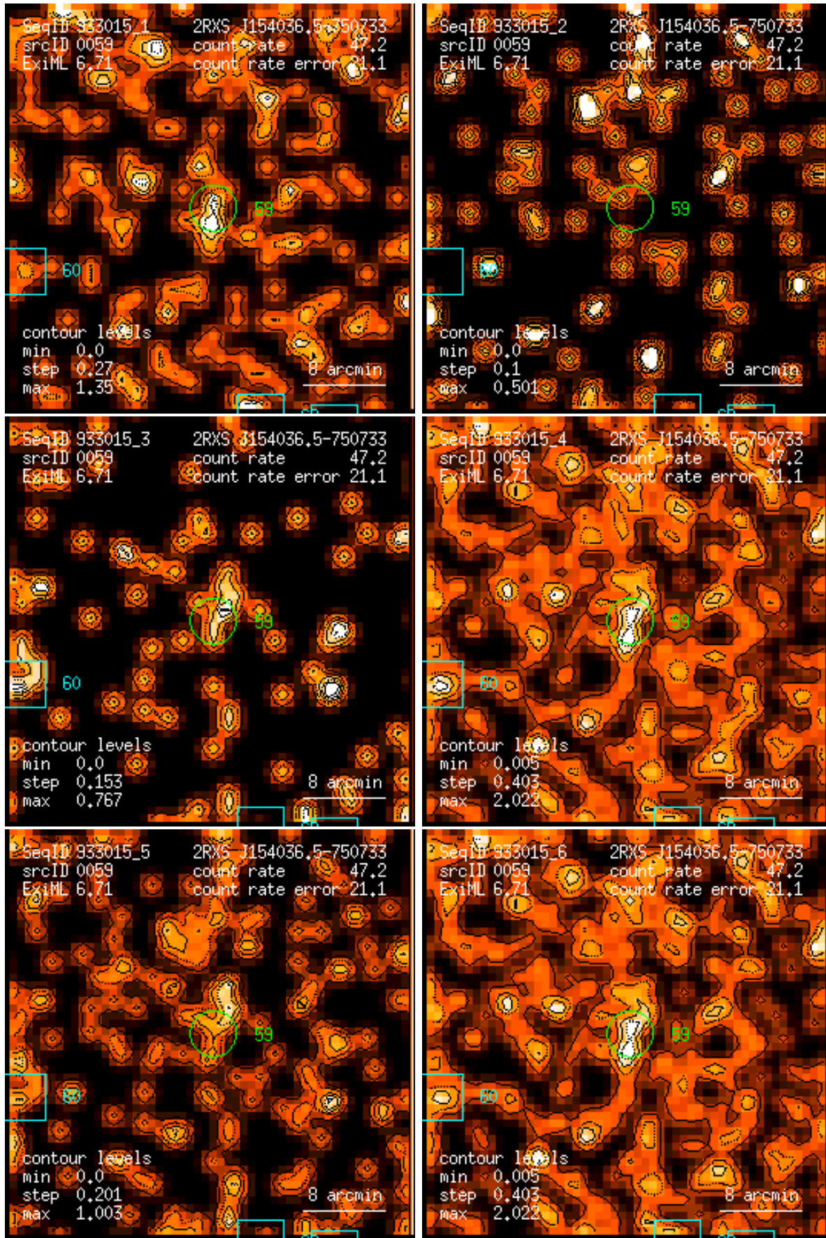
Figure 59: RASS 933015: detection 0059: band rate images, Gaussian filter: (1) PSPC channels 11 – 41, (2) 52 – 90, (3) 91 – 201, (4) 11 – 235, (5) 52 – 201, (6) 11 – 201. Broad band rates in counts/ks. Band rate contour levels in counts/ks/arcmin 2 .
