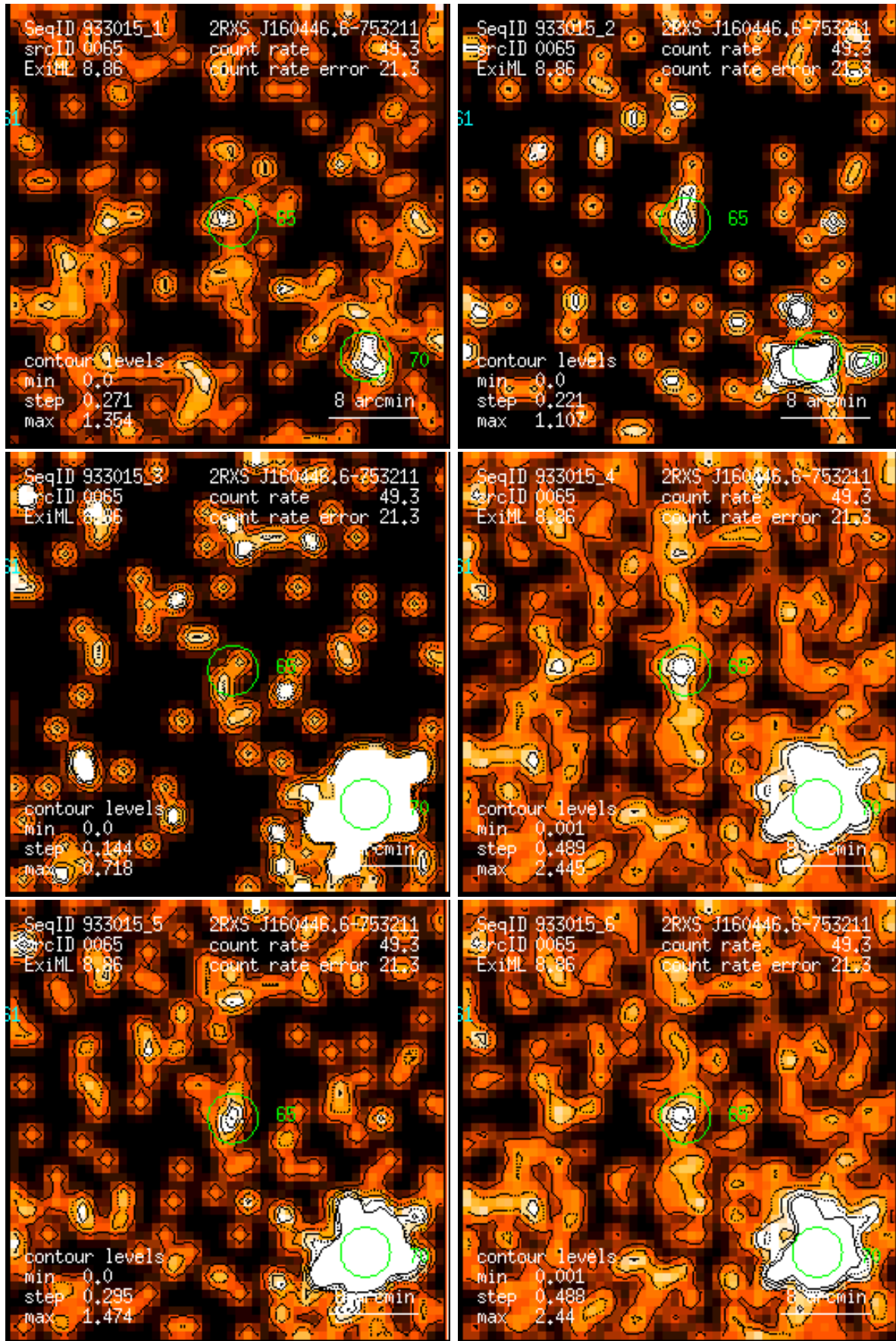
Figure 65: RASS 933015: detection 0065: band rate images, Gaussian filter: (1) PSPC channels 11 – 41, (2) 52 – 90, (3) 91 – 201, (4) 11 – 235, (5) 52 – 201, (6) 11 – 201. Broad band rates in counts/ks. Band rate contour levels in counts/ks/arcmin 2 .
