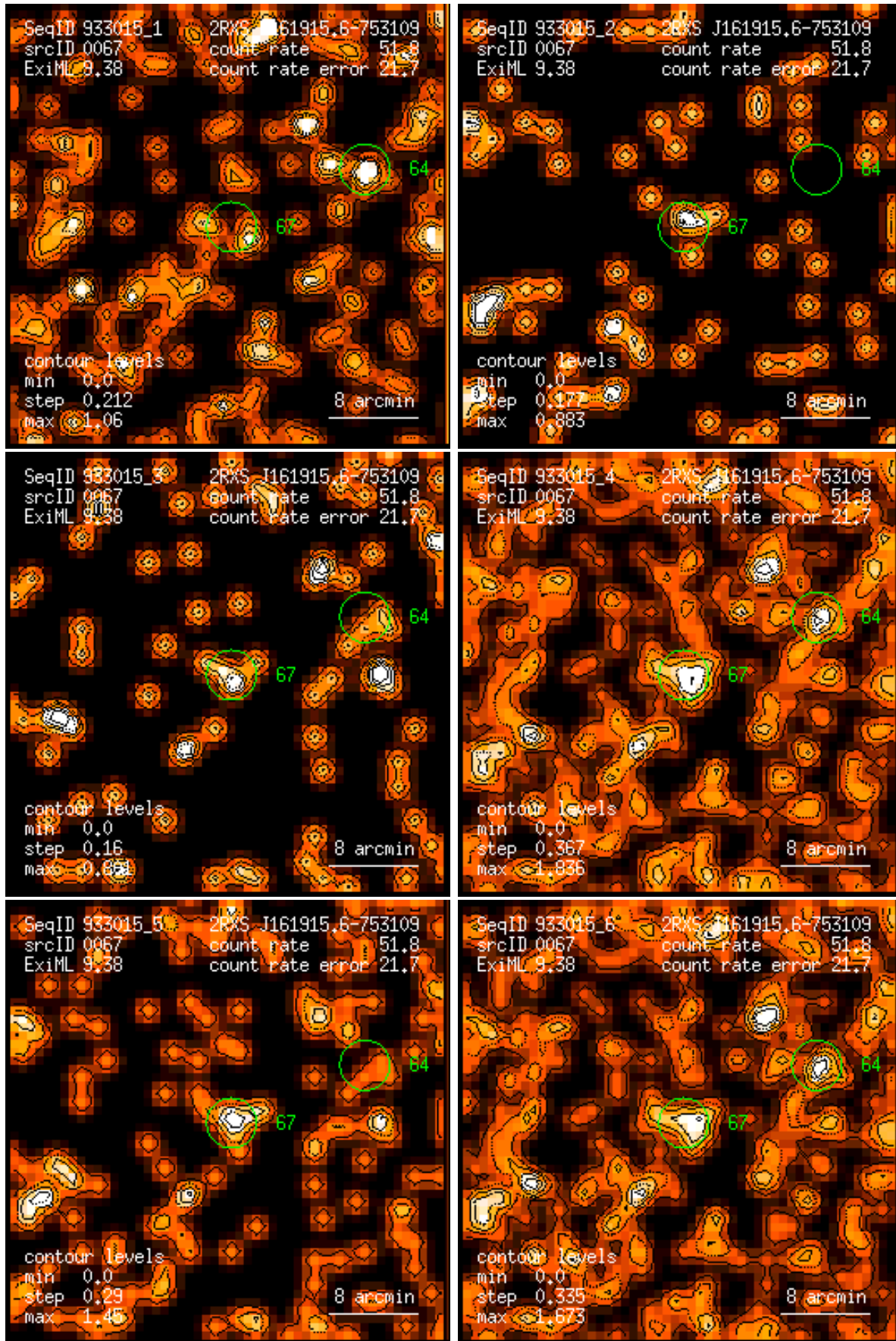
Figure 67: RASS 933015: detection 0067: band rate images, Gaussian filter: (1) PSPC channels 11 – 41, (2) 52 – 90, (3) 91 – 201, (4) 11 – 235, (5) 52 – 201, (6) 11 – 201. Broad band rates in counts/ks. Band rate contour levels in counts/ks/arcmin 2 .
