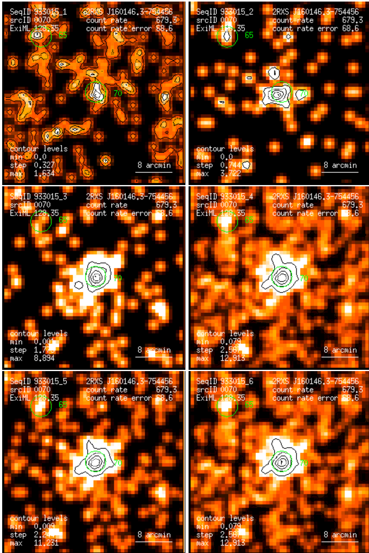
Figure 70: RASS 933015: detection 0070: band rate images, Gaussian filter: (1) PSPC channels 11 – 41, (2) 52 – 90, (3) 91 – 201, (4) 11 – 235, (5) 52 – 201, (6) 11 – 201. Broad band rates in counts/ks. Band rate contour levels in counts/ks/arcmin 2 .
