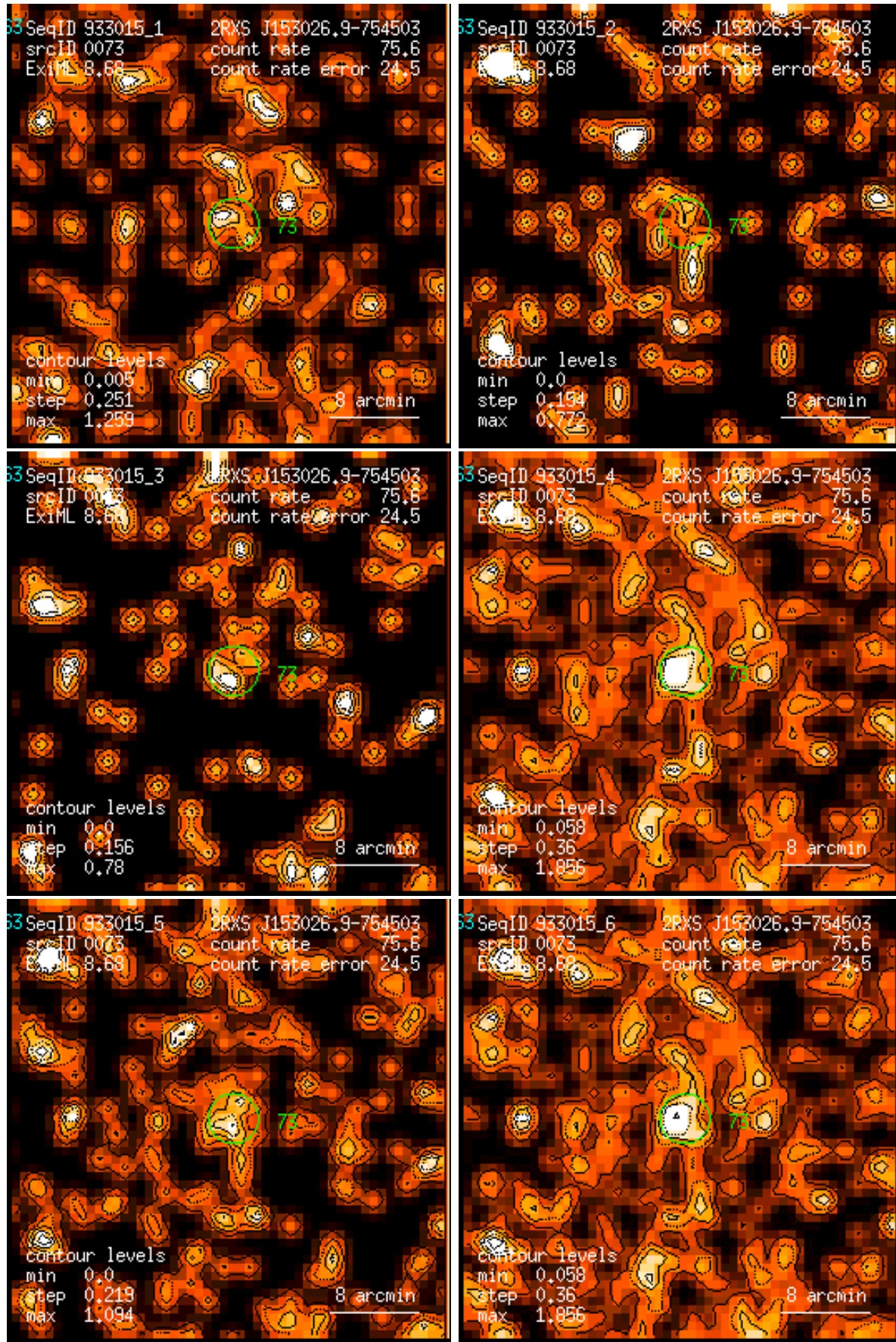
Figure 73: RASS 933015: detection 0073: band rate images, Gaussian filter: (1) PSPC channels 11 – 41, (2) 52 – 90, (3) 91 – 201, (4) 11 – 235, (5) 52 – 201, (6) 11 – 201. Broad band rates in counts/ks. Band rate contour levels in counts/ks/arcmin 2 .
