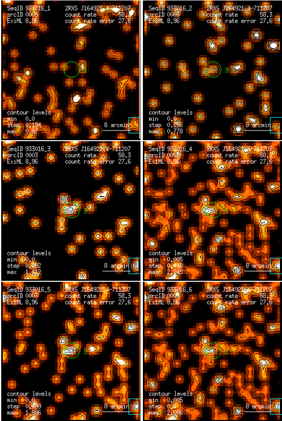
Figure 3: RASS 933016: detection 0003: band rate images, Gaussian filter: (1) PSPC channels 11 – 41, (2) 52 – 90, (3) 91 – 201, (4) 11 – 235, (5) 52 – 201, (6) 11 – 201. Broad band rates in counts/ks. Band rate contour levels in counts/ks/arcmin 2 .
