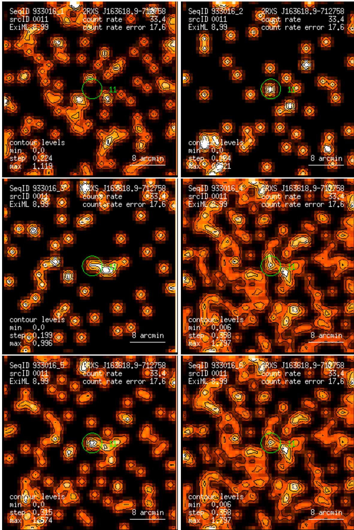
Figure 11: RASS 933016: detection 0011: band rate images, Gaussian filter: (1) PSPC channels 11 – 41, (2) 52 – 90, (3) 91 – 201, (4) 11 – 235, (5) 52 – 201, (6) 11 – 201. Broad band rates in counts/ks. Band rate contour levels in counts/ks/arcmin 2 .
