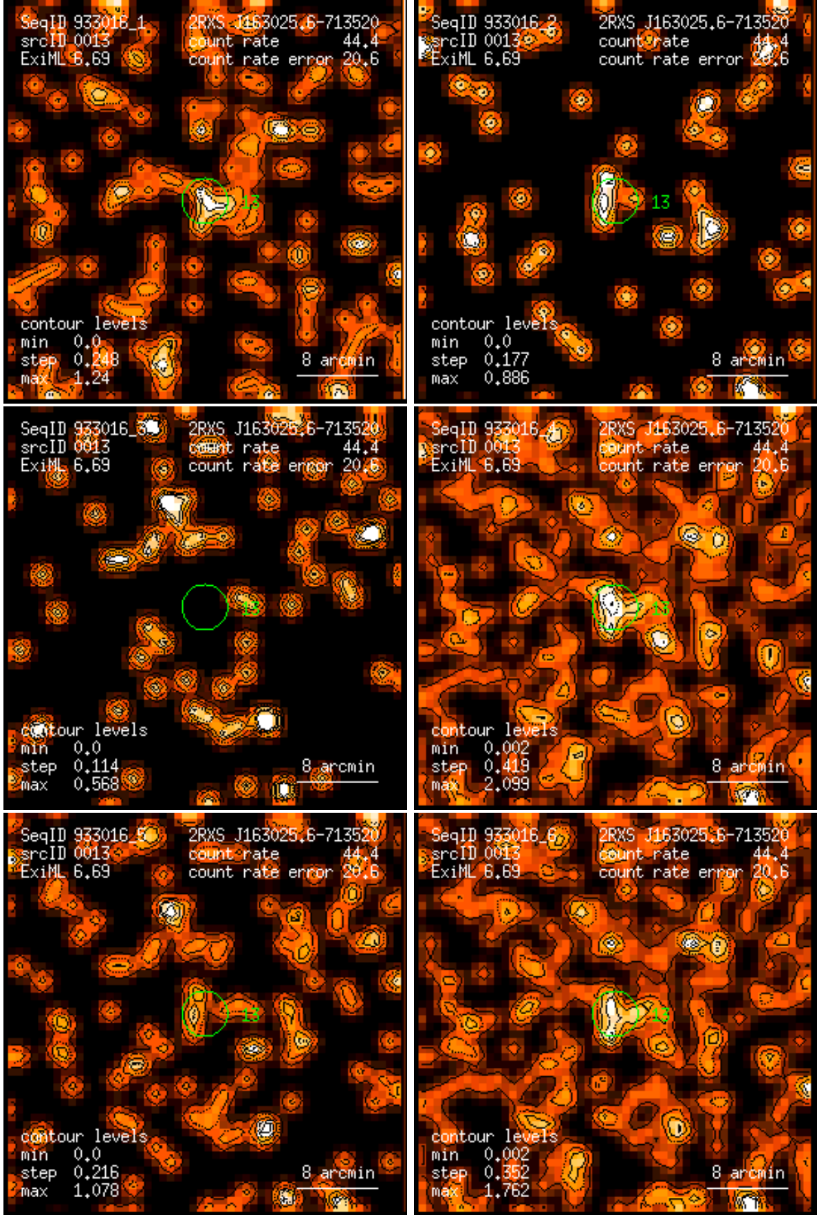
Figure 13: RASS 933016: detection 0013: band rate images, Gaussian filter: (1) PSPC channels 11 – 41, (2) 52 – 90, (3) 91 – 201, (4) 11 – 235, (5) 52 – 201, (6) 11 – 201. Broad band rates in counts/ks. Band rate contour levels in counts/ks/arcmin 2 .
