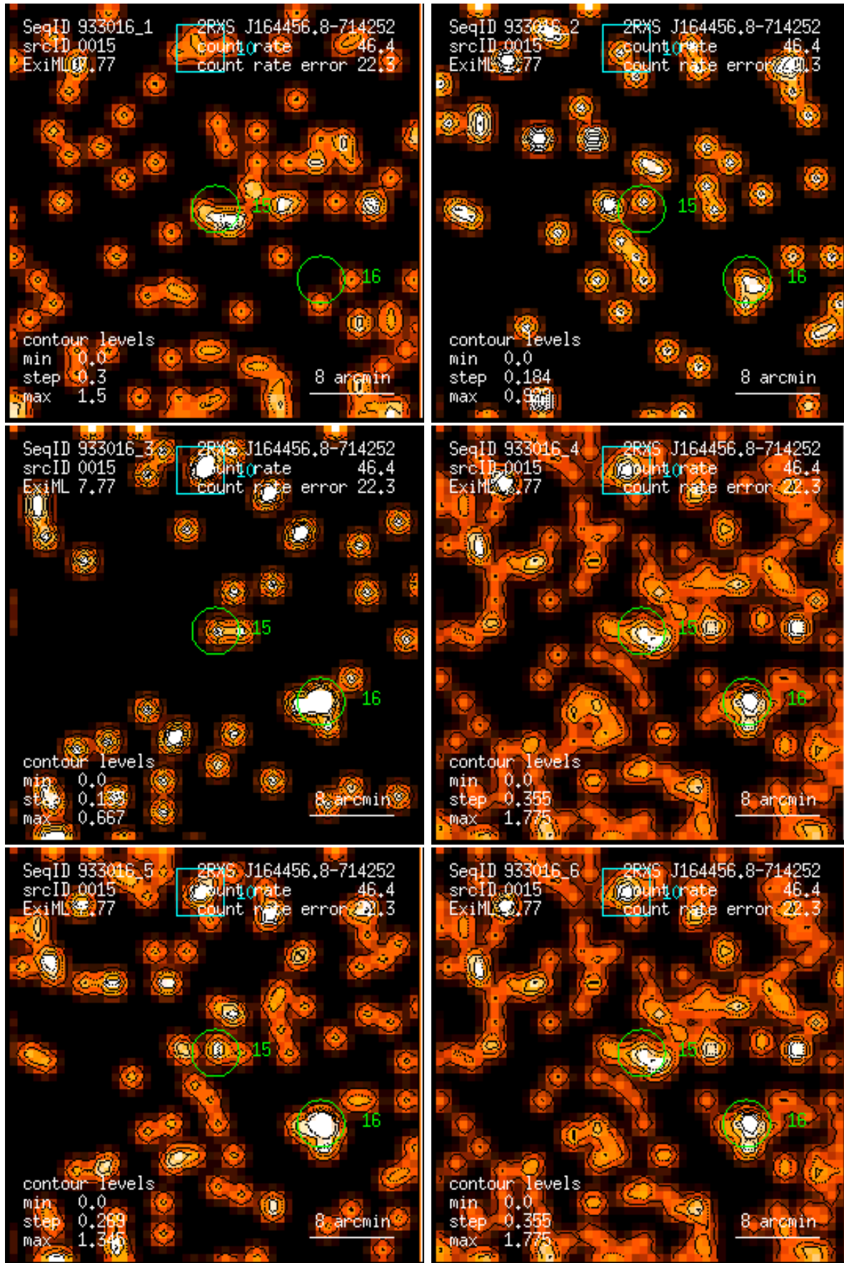
Figure 15: RASS 933016: detection 0015: band rate images, Gaussian filter: (1) PSPC channels 11 – 41, (2) 52 – 90, (3) 91 – 201, (4) 11 – 235, (5) 52 – 201, (6) 11 – 201. Broad band rates in counts/ks. Band rate contour levels in counts/ks/arcmin 2 .
