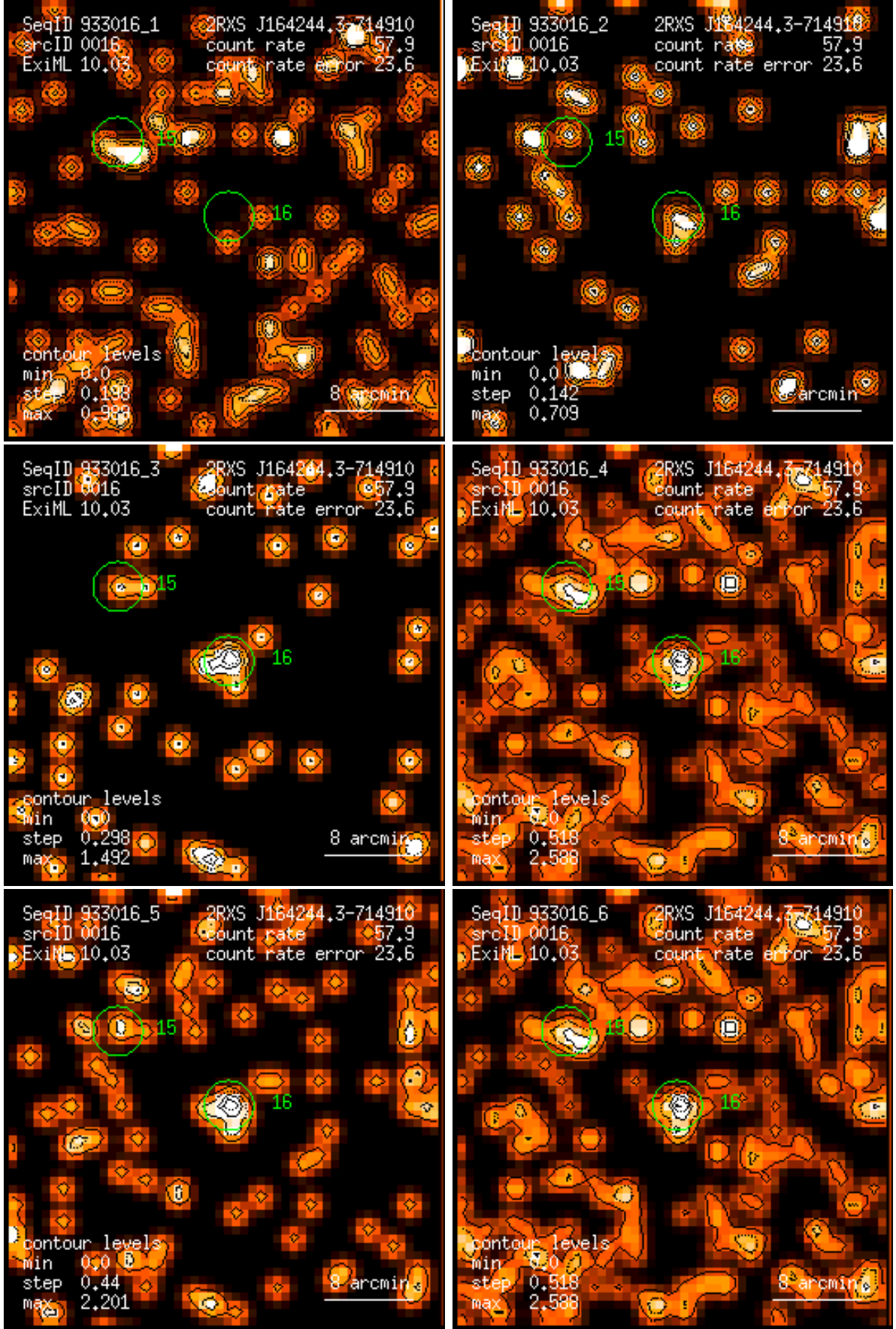
Figure 16: RASS 933016: detection 0016: band rate images, Gaussian filter: (1) PSPC channels 11 – 41, (2) 52 – 90, (3) 91 – 201, (4) 11 – 235, (5) 52 – 201, (6) 11 – 201. Broad band rates in counts/ks. Band rate contour levels in counts/ks/arcmin 2 .
