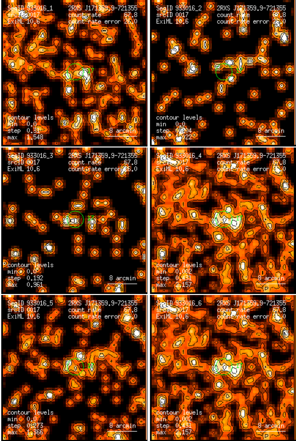
Figure 17: RASS 933016: detection 0017: band rate images, Gaussian filter: (1) PSPC channels 11 – 41, (2) 52 – 90, (3) 91 – 201, (4) 11 – 235, (5) 52 – 201, (6) 11 – 201. Broad band rates in counts/ks. Band rate contour levels in counts/ks/arcmin 2 .
