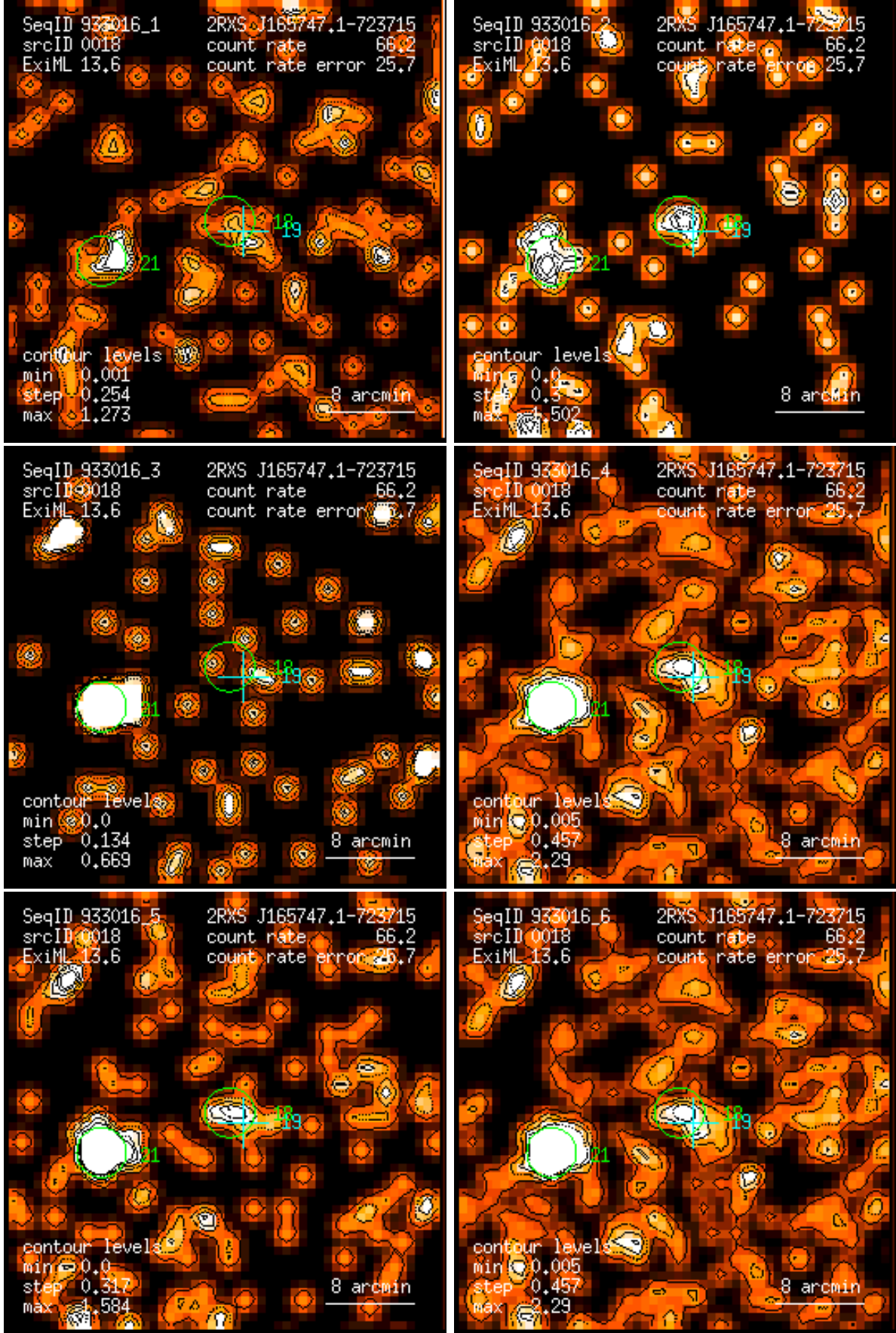
Figure 18: RASS 933016: detection 0018: band rate images, Gaussian filter: (1) PSPC channels 11 – 41, (2) 52 – 90, (3) 91 – 201, (4) 11 – 235, (5) 52 – 201, (6) 11 – 201. Broad band rates in counts/ks. Band rate contour levels in counts/ks/arcmin 2 .
