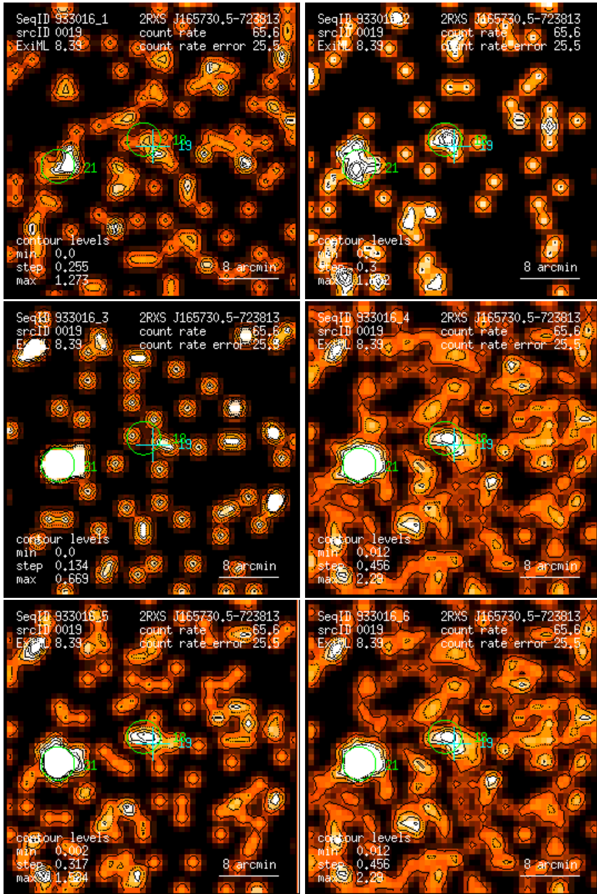
Figure 19: RASS 933016: detection 0019: band rate images, Gaussian filter: (1) PSPC channels 11 – 41, (2) 52 – 90, (3) 91 – 201, (4) 11 – 235, (5) 52 – 201, (6) 11 – 201. Broad band rates in counts/ks. Band rate contour levels in counts/ks/arcmin 2 .
