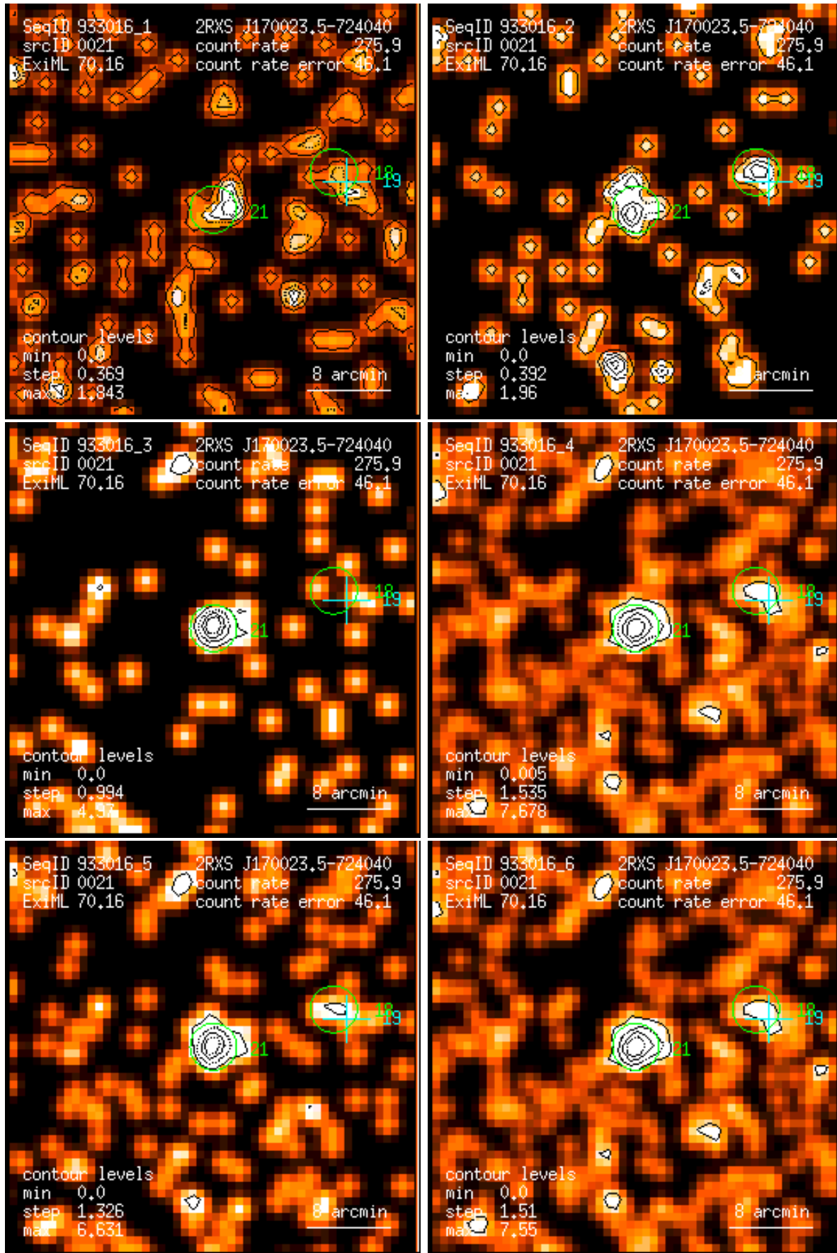
Figure 21: RASS 933016: detection 0021: band rate images, Gaussian filter: (1) PSPC channels 11 – 41, (2) 52 – 90, (3) 91 – 201, (4) 11 – 235, (5) 52 – 201, (6) 11 – 201. Broad band rates in counts/ks. Band rate contour levels in counts/ks/arcmin 2 .
