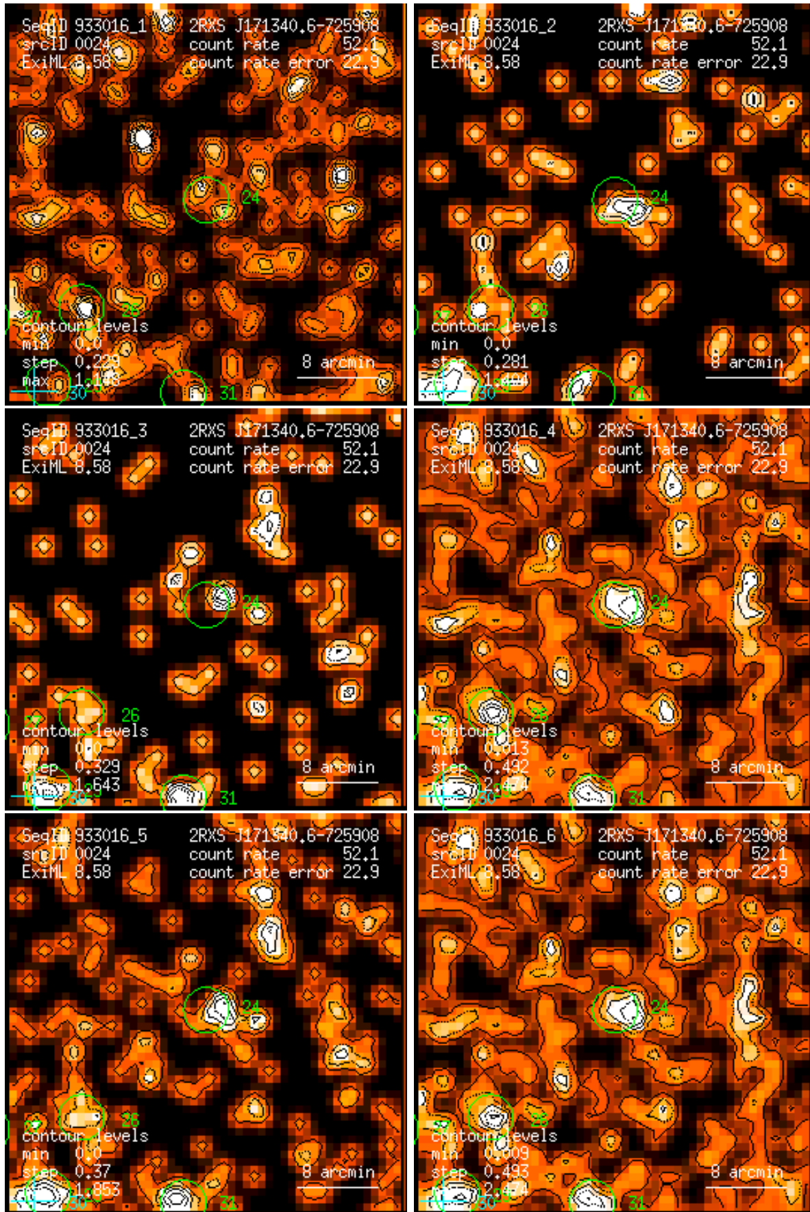
Figure 24: RASS 933016: detection 0024: band rate images, Gaussian filter: (1) PSPC channels 11 – 41, (2) 52 – 90, (3) 91 – 201, (4) 11 – 235, (5) 52 – 201, (6) 11 – 201. Broad band rates in counts/ks. Band rate contour levels in counts/ks/arcmin 2 .
