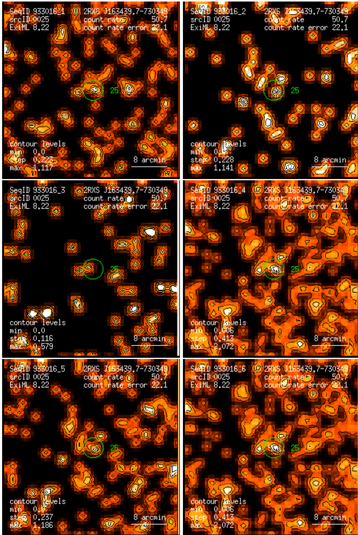
Figure 25: RASS 933016: detection 0025: band rate images, Gaussian filter: (1) PSPC channels 11 – 41, (2) 52 – 90, (3) 91 – 201, (4) 11 – 235, (5) 52 – 201, (6) 11 – 201. Broad band rates in counts/ks. Band rate contour levels in counts/ks/arcmin 2 .
