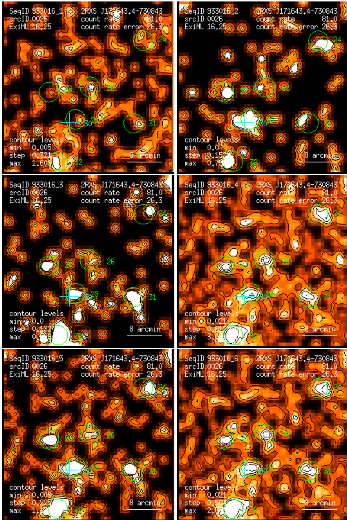
Figure 26: RASS 933016: detection 0026: band rate images, Gaussian filter: (1) PSPC channels 11 – 41, (2) 52 – 90, (3) 91 – 201, (4) 11 – 235, (5) 52 – 201, (6) 11 – 201. Broad band rates in counts/ks. Band rate contour levels in counts/ks/arcmin 2 .
