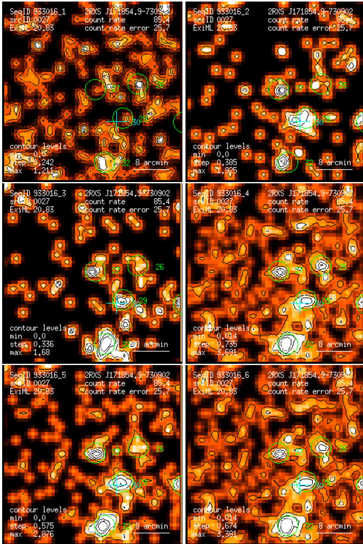
Figure 27: RASS 933016: detection 0027: band rate images, Gaussian filter: (1) PSPC channels 11 – 41, (2) 52 – 90, (3) 91 – 201, (4) 11 – 235, (5) 52 – 201, (6) 11 – 201. Broad band rates in counts/ks. Band rate contour levels in counts/ks/arcmin 2 .
