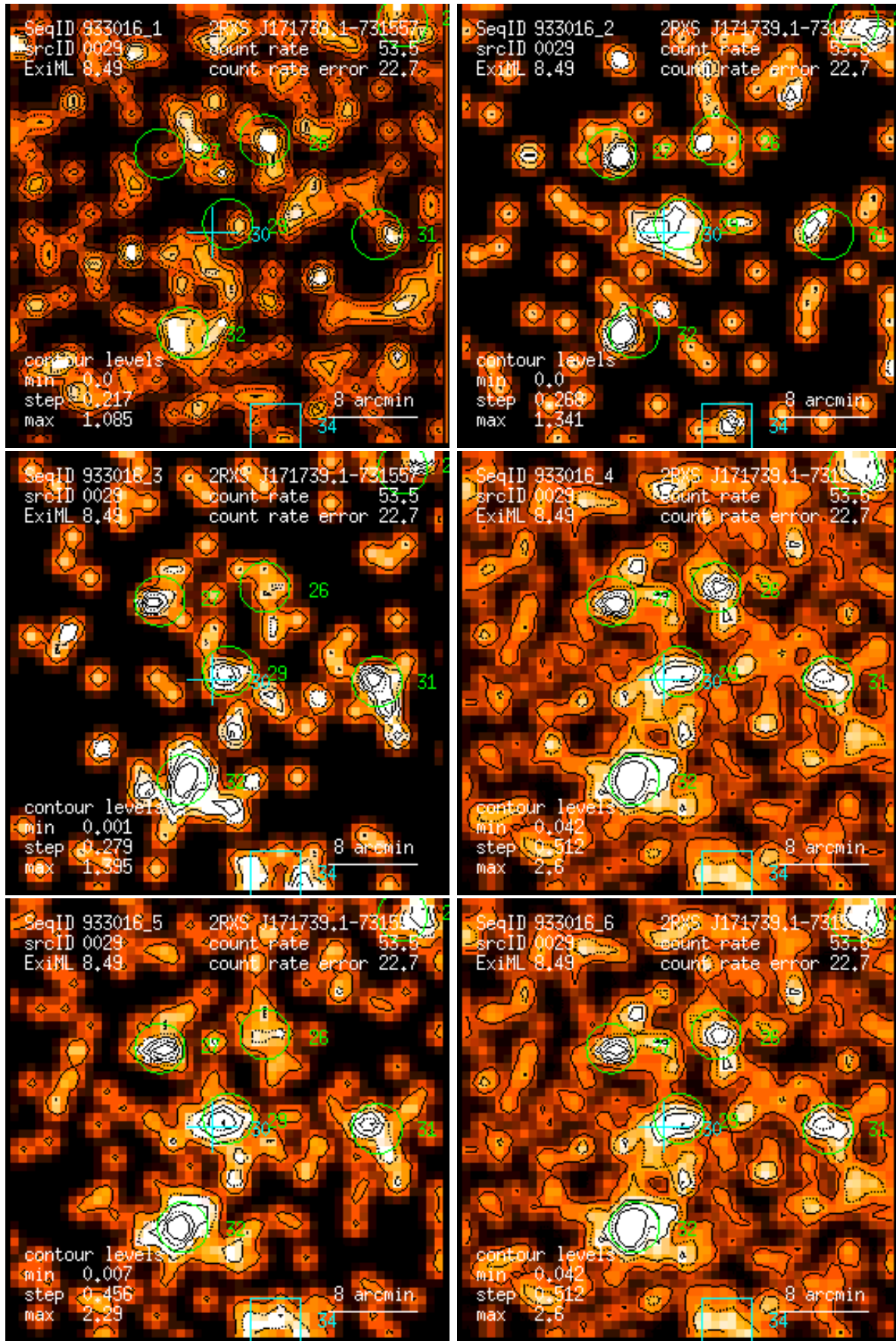
Figure 29: RASS 933016: detection 0029: band rate images, Gaussian filter: (1) PSPC channels 11 – 41, (2) 52 – 90, (3) 91 – 201, (4) 11 – 235, (5) 52 – 201, (6) 11 – 201. Broad band rates in counts/ks. Band rate contour levels in counts/ks/arcmin 2 .
