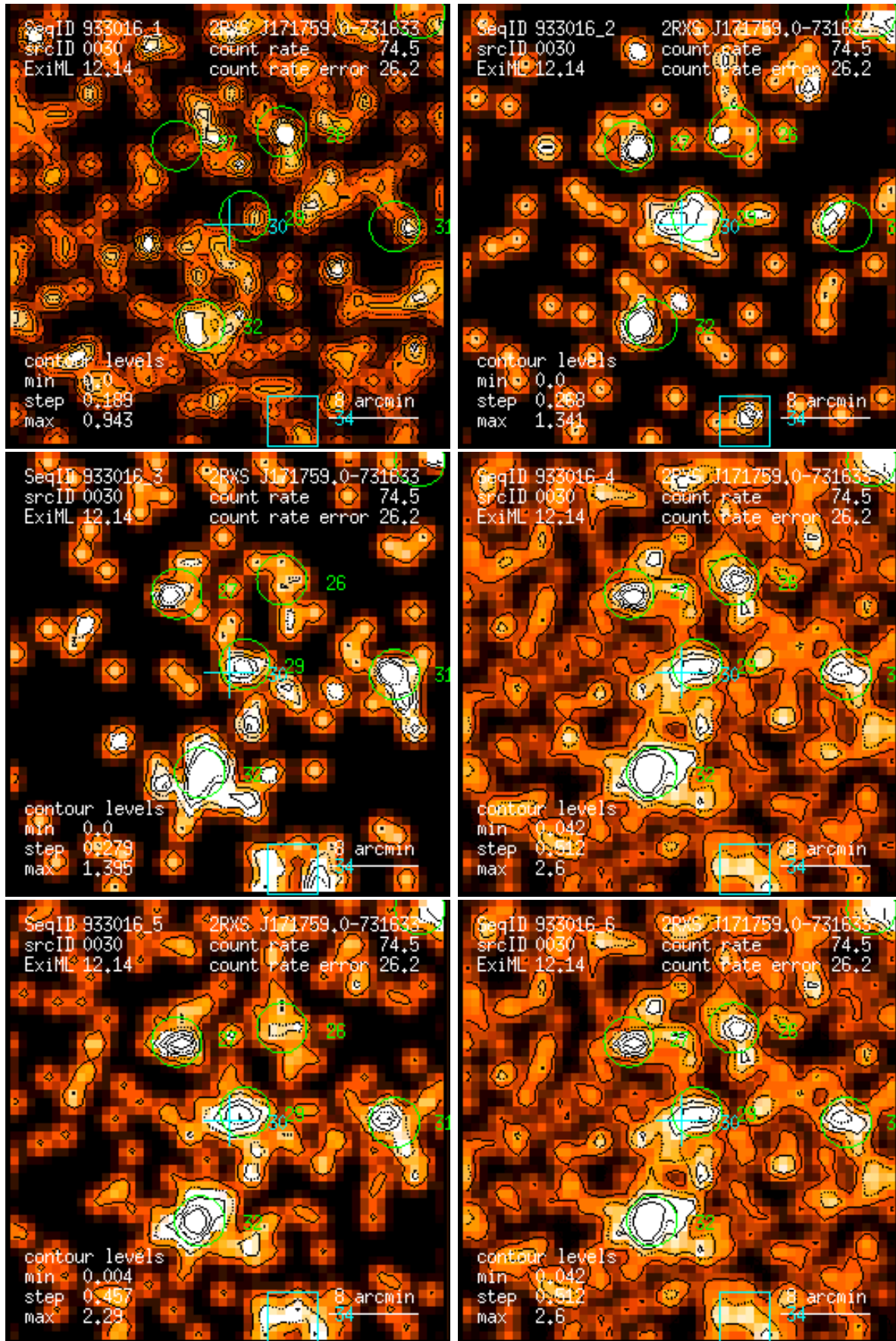
Figure 30: RASS 933016: detection 0030: band rate images, Gaussian filter: (1) PSPC channels 11 – 41, (2) 52 – 90, (3) 91 – 201, (4) 11 – 235, (5) 52 – 201, (6) 11 – 201. Broad band rates in counts/ks. Band rate contour levels in counts/ks/arcmin 2 .
