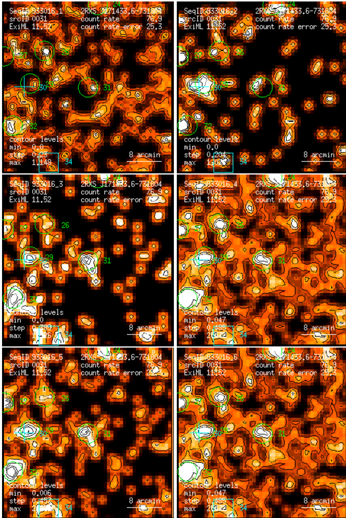
Figure 31: RASS 933016: detection 0031: band rate images, Gaussian filter: (1) PSPC channels 11 – 41, (2) 52 – 90, (3) 91 – 201, (4) 11 – 235, (5) 52 – 201, (6) 11 – 201. Broad band rates in counts/ks. Band rate contour levels in counts/ks/arcmin 2 .
