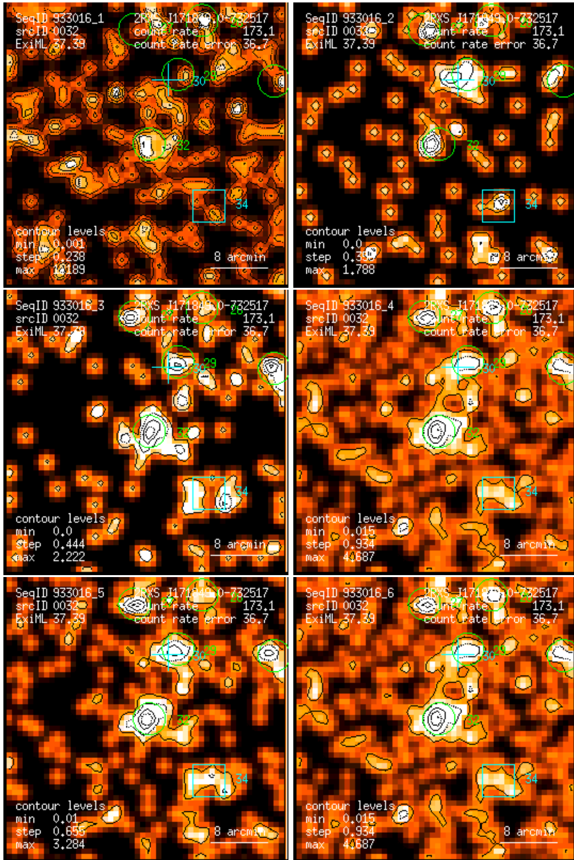
Figure 32: RASS 933016: detection 0032: band rate images, Gaussian filter: (1) PSPC channels 11 – 41, (2) 52 – 90, (3) 91 – 201, (4) 11 – 235, (5) 52 – 201, (6) 11 – 201. Broad band rates in counts/ks. Band rate contour levels in counts/ks/arcmin 2 .
