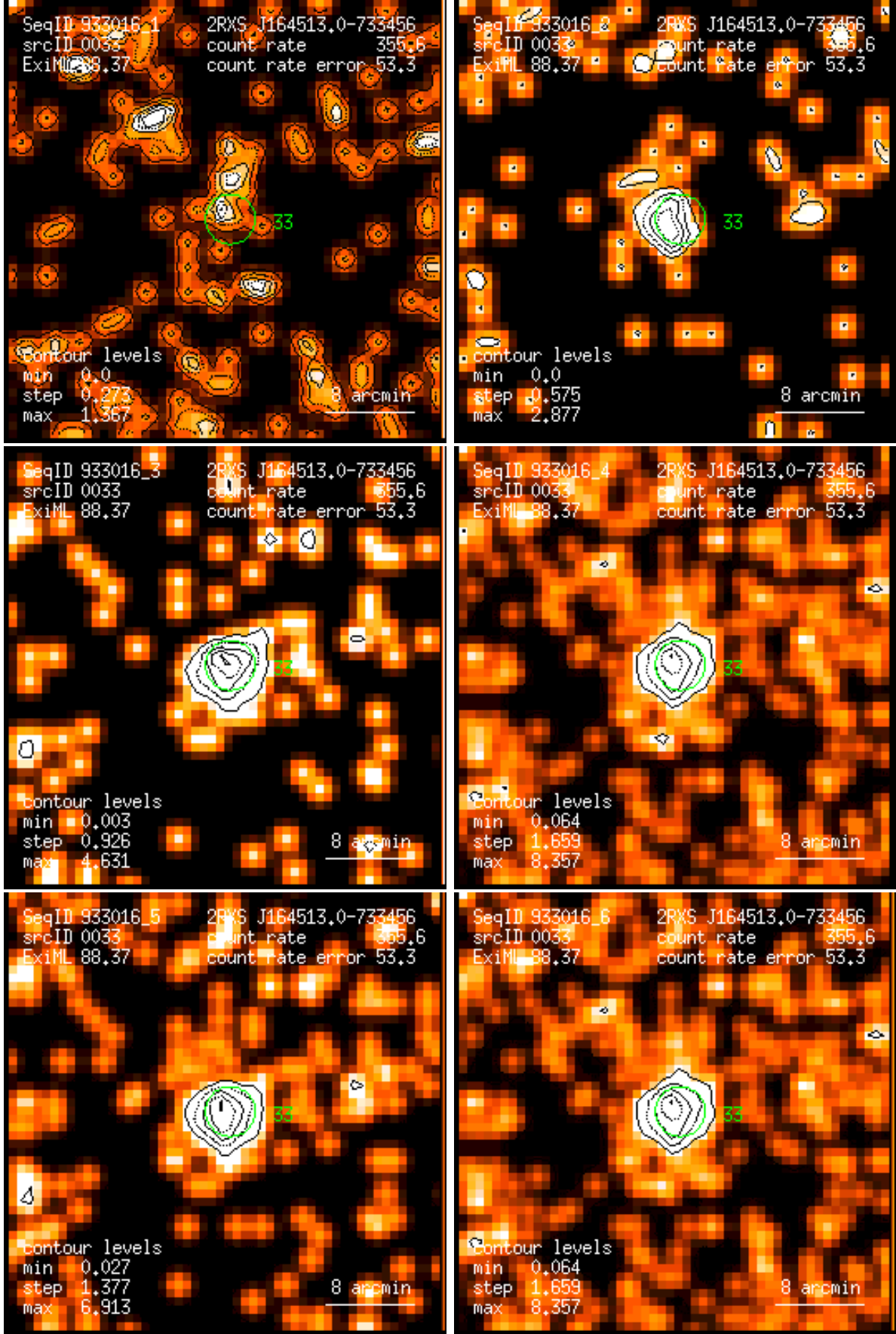
Figure 33: RASS 933016: detection 0033: band rate images, Gaussian filter: (1) PSPC channels 11 – 41, (2) 52 – 90, (3) 91 – 201, (4) 11 – 235, (5) 52 – 201, (6) 11 – 201. Broad band rates in counts/ks. Band rate contour levels in counts/ks/arcmin 2 .
