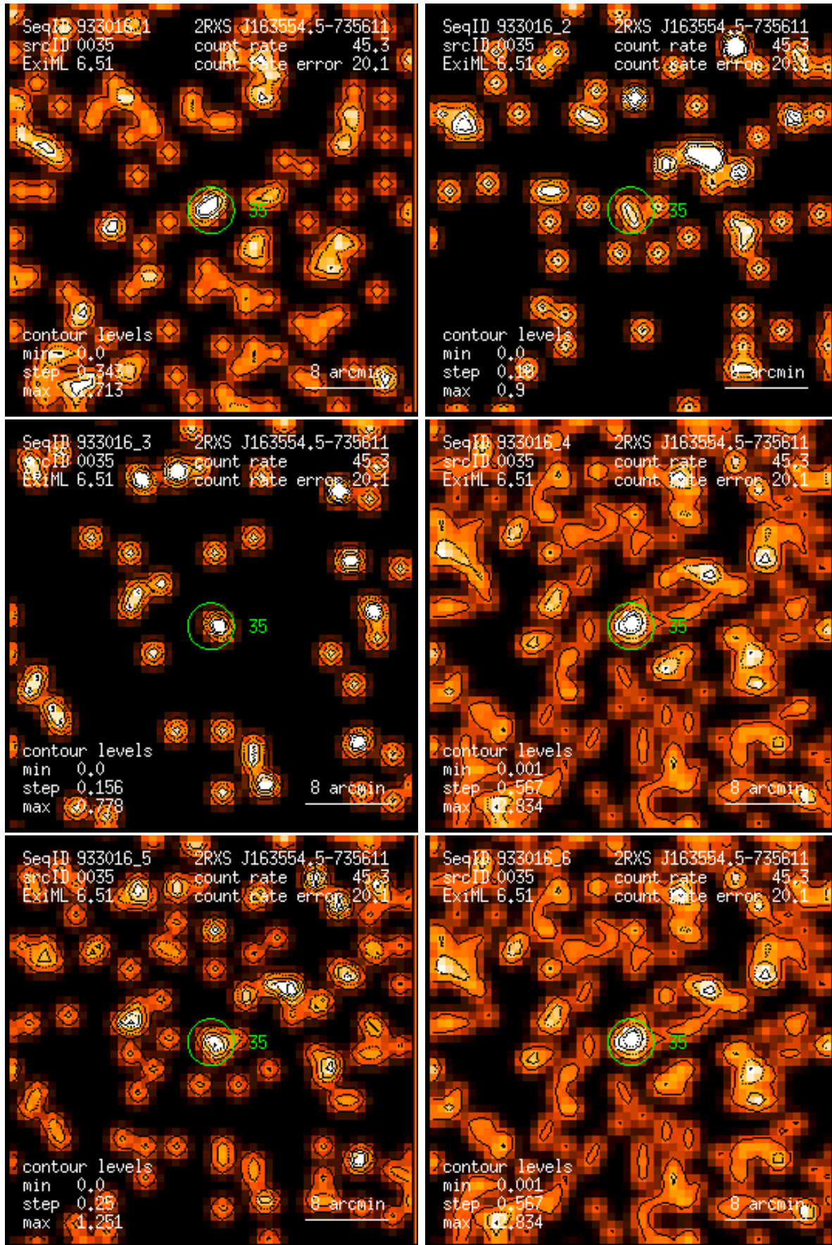
Figure 35: RASS 933016: detection 0035: band rate images, Gaussian filter: (1) PSPC channels 11 – 41, (2) 52 – 90, (3) 91 – 201, (4) 11 – 235, (5) 52 – 201, (6) 11 – 201. Broad band rates in counts/ks. Band rate contour levels in counts/ks/arcmin 2 .
