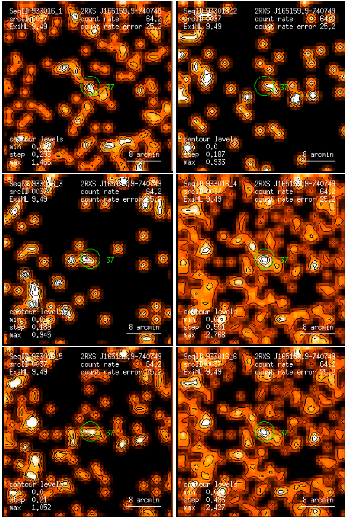
Figure 37: RASS 933016: detection 0037: band rate images, Gaussian filter: (1) PSPC channels 11 – 41, (2) 52 – 90, (3) 91 – 201, (4) 11 – 235, (5) 52 – 201, (6) 11 – 201. Broad band rates in counts/ks. Band rate contour levels in counts/ks/arcmin 2 .
