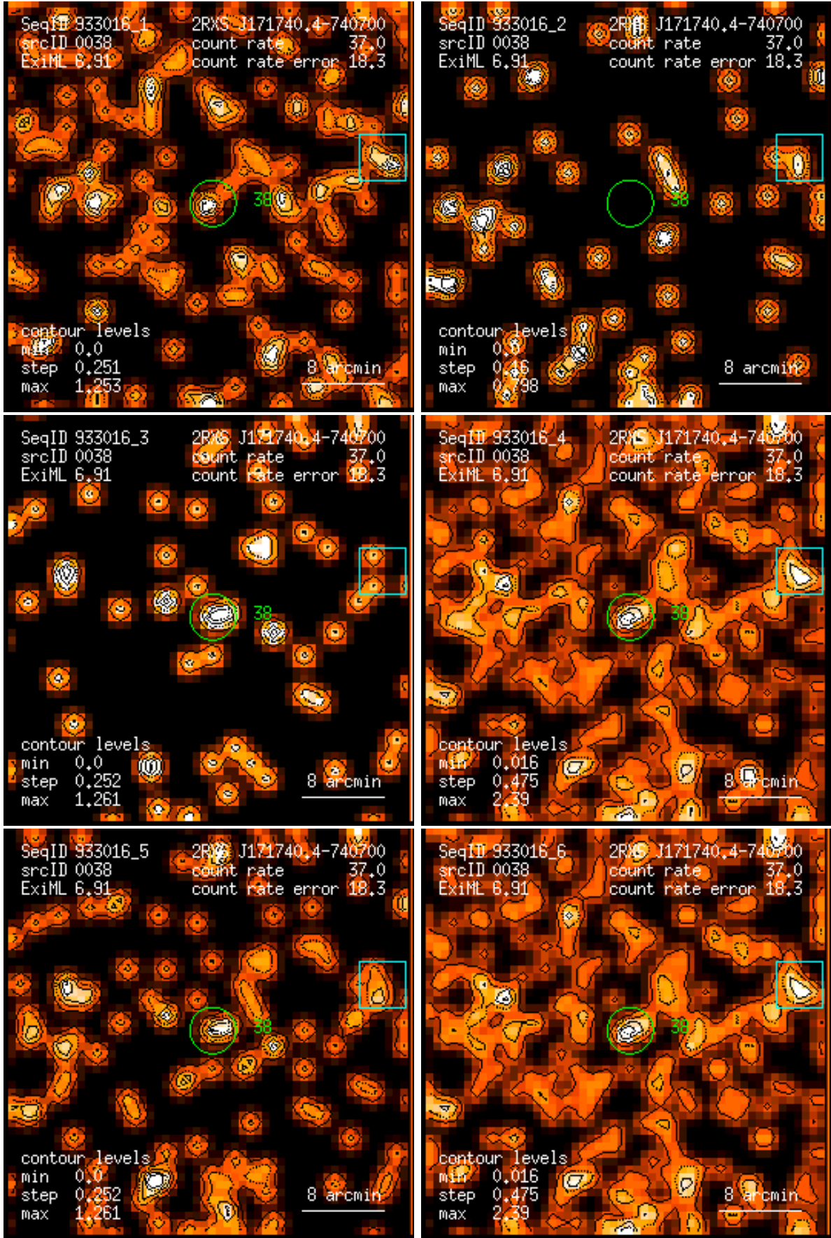
Figure 38: RASS 933016: detection 0038: band rate images, Gaussian filter: (1) PSPC channels 11 – 41, (2) 52 – 90, (3) 91 – 201, (4) 11 – 235, (5) 52 – 201, (6) 11 – 201. Broad band rates in counts/ks. Band rate contour levels in counts/ks/arcmin 2 .
