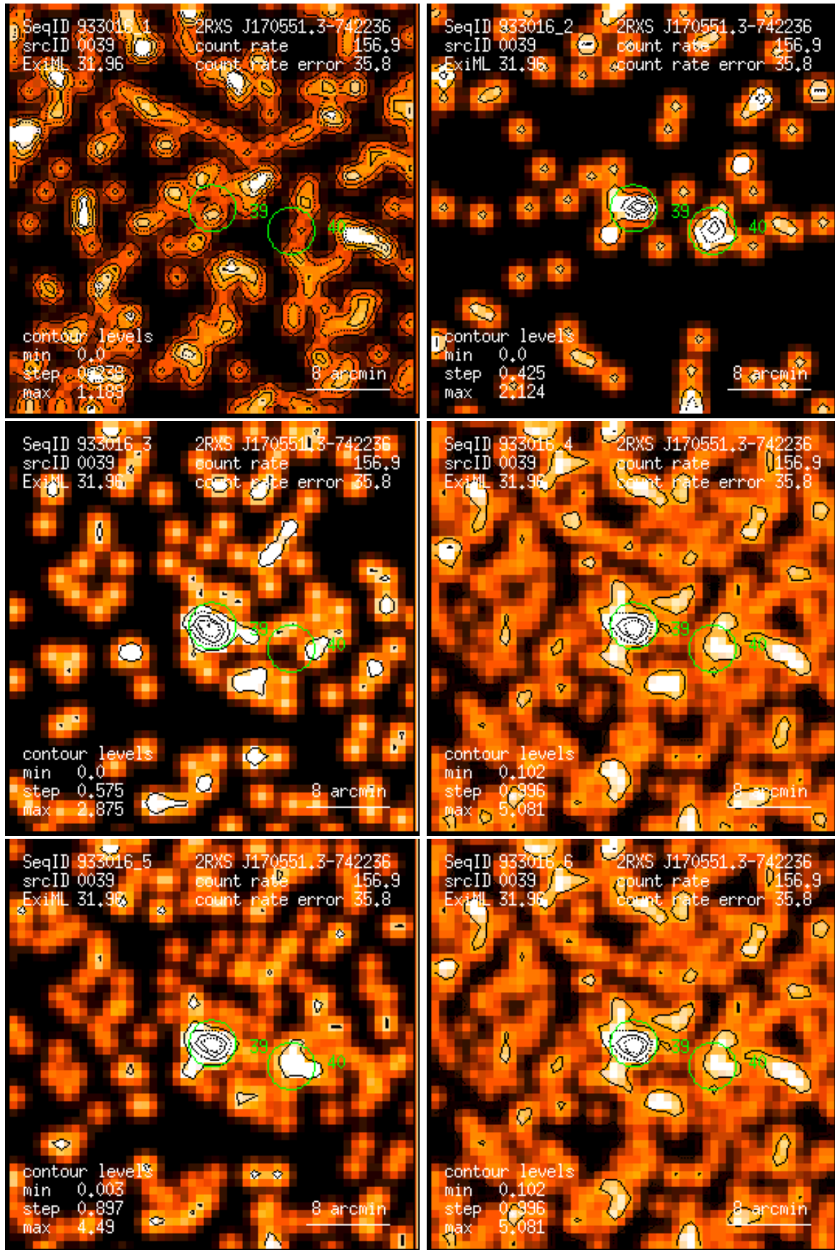
Figure 39: RASS 933016: detection 0039: band rate images, Gaussian filter: (1) PSPC channels 11 – 41, (2) 52 – 90, (3) 91 – 201, (4) 11 – 235, (5) 52 – 201, (6) 11 – 201. Broad band rates in counts/ks. Band rate contour levels in counts/ks/arcmin 2 .
