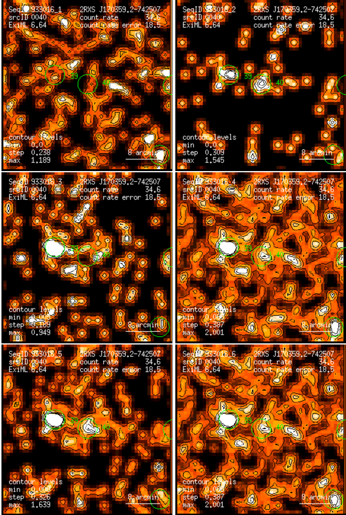
Figure 40: RASS 933016: detection 0040: band rate images, Gaussian filter: (1) PSPC channels 11 – 41, (2) 52 – 90, (3) 91 – 201, (4) 11 – 235, (5) 52 – 201, (6) 11 – 201. Broad band rates in counts/ks. Band rate contour levels in counts/ks/arcmin 2 .
