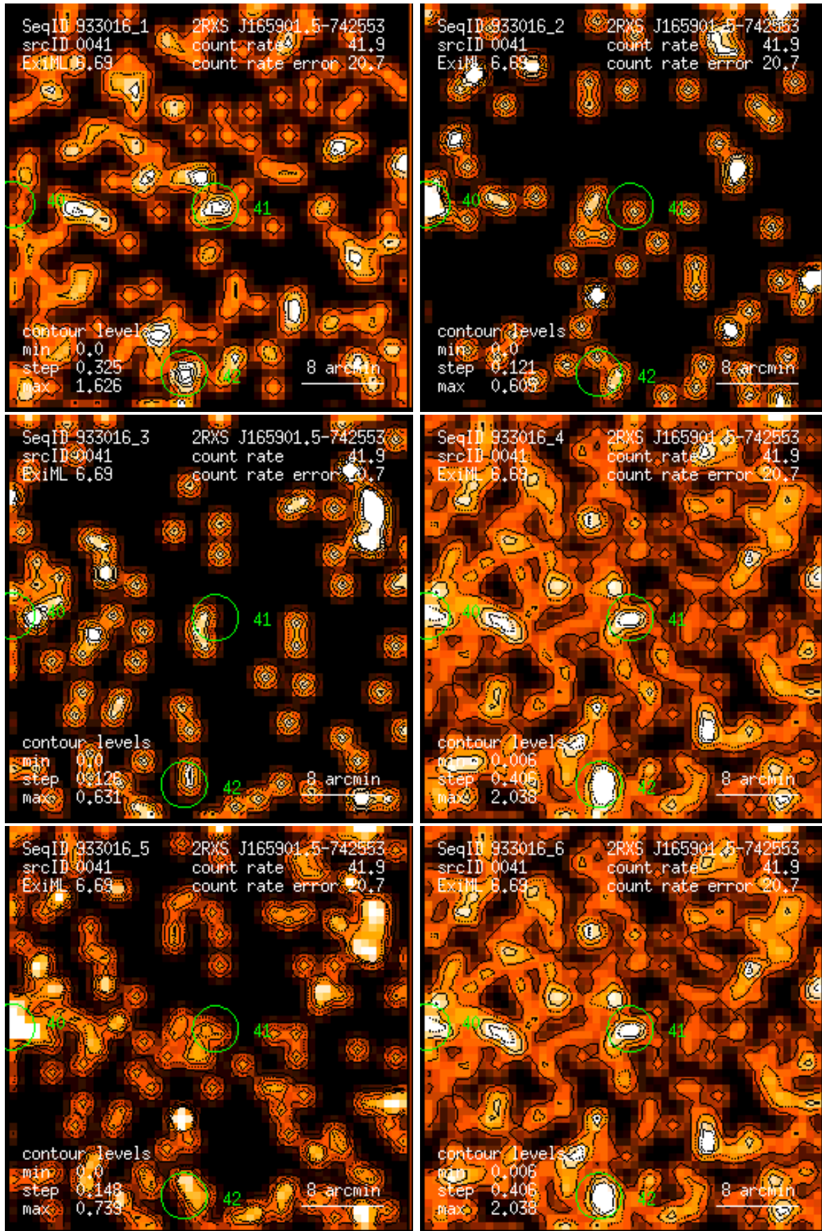
Figure 41: RASS 933016: detection 0041: band rate images, Gaussian filter: (1) PSPC channels 11 – 41, (2) 52 – 90, (3) 91 – 201, (4) 11 – 235, (5) 52 – 201, (6) 11 – 201. Broad band rates in counts/ks. Band rate contour levels in counts/ks/arcmin 2 .
