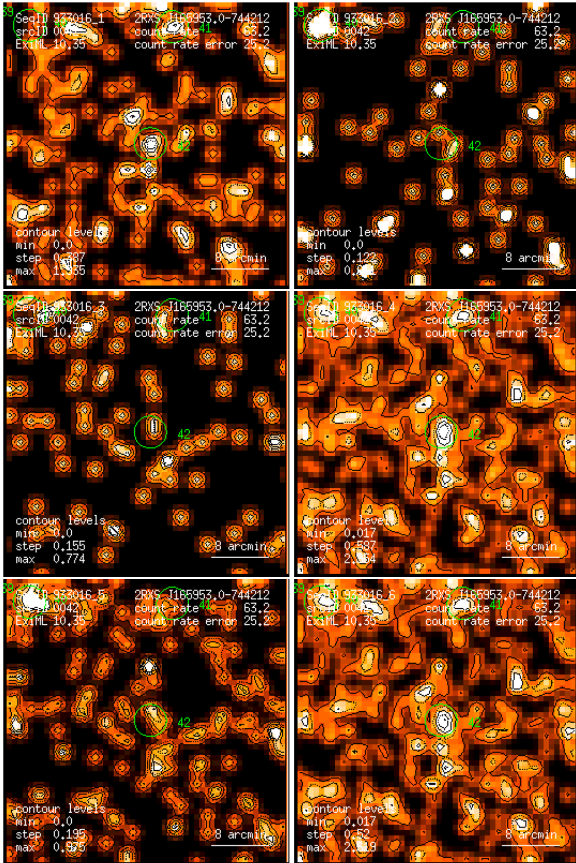
Figure 42: RASS 933016: detection 0042: band rate images, Gaussian filter: (1) PSPC channels 11 – 41, (2) 52 – 90, (3) 91 – 201, (4) 11 – 235, (5) 52 – 201, (6) 11 – 201. Broad band rates in counts/ks. Band rate contour levels in counts/ks/arcmin 2 .
