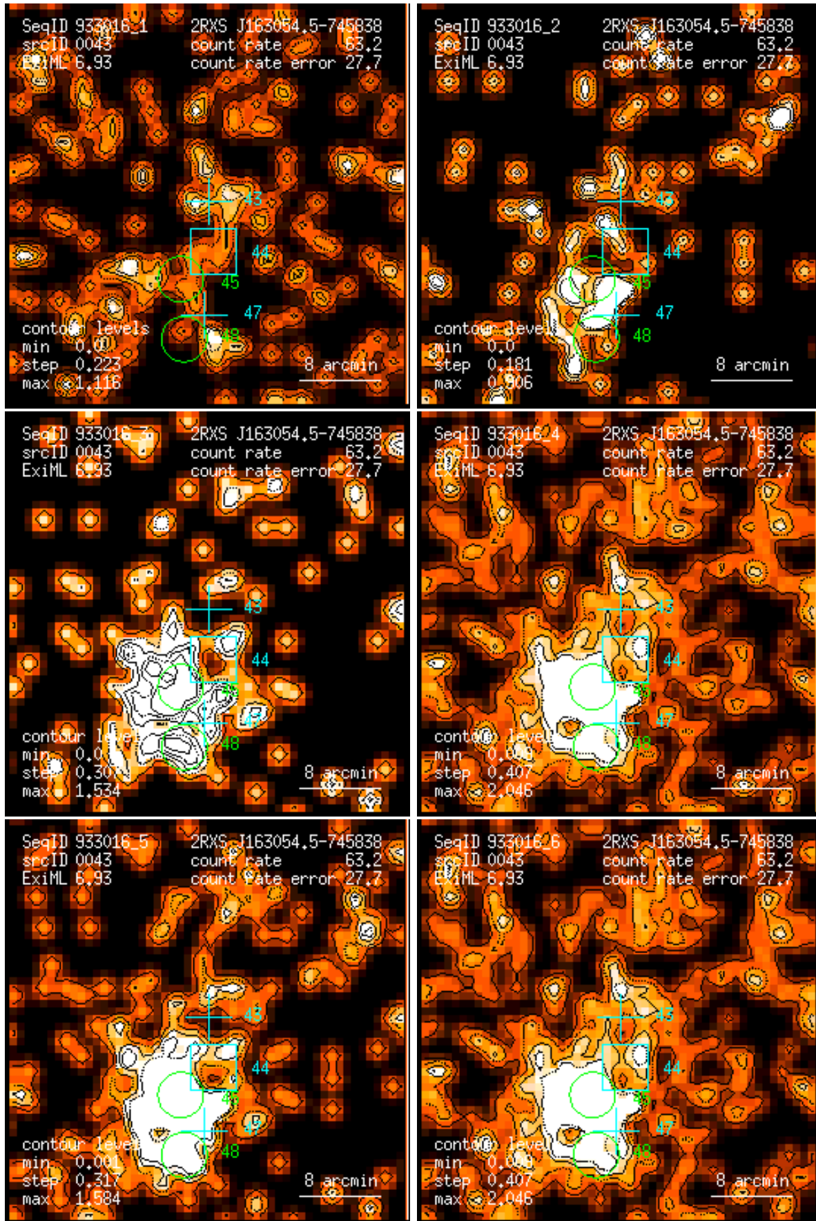
Figure 43: RASS 933016: detection 0043: band rate images, Gaussian filter: (1) PSPC channels 11 – 41, (2) 52 – 90, (3) 91 – 201, (4) 11 – 235, (5) 52 – 201, (6) 11 – 201. Broad band rates in counts/ks. Band rate contour levels in counts/ks/arcmin 2 .
