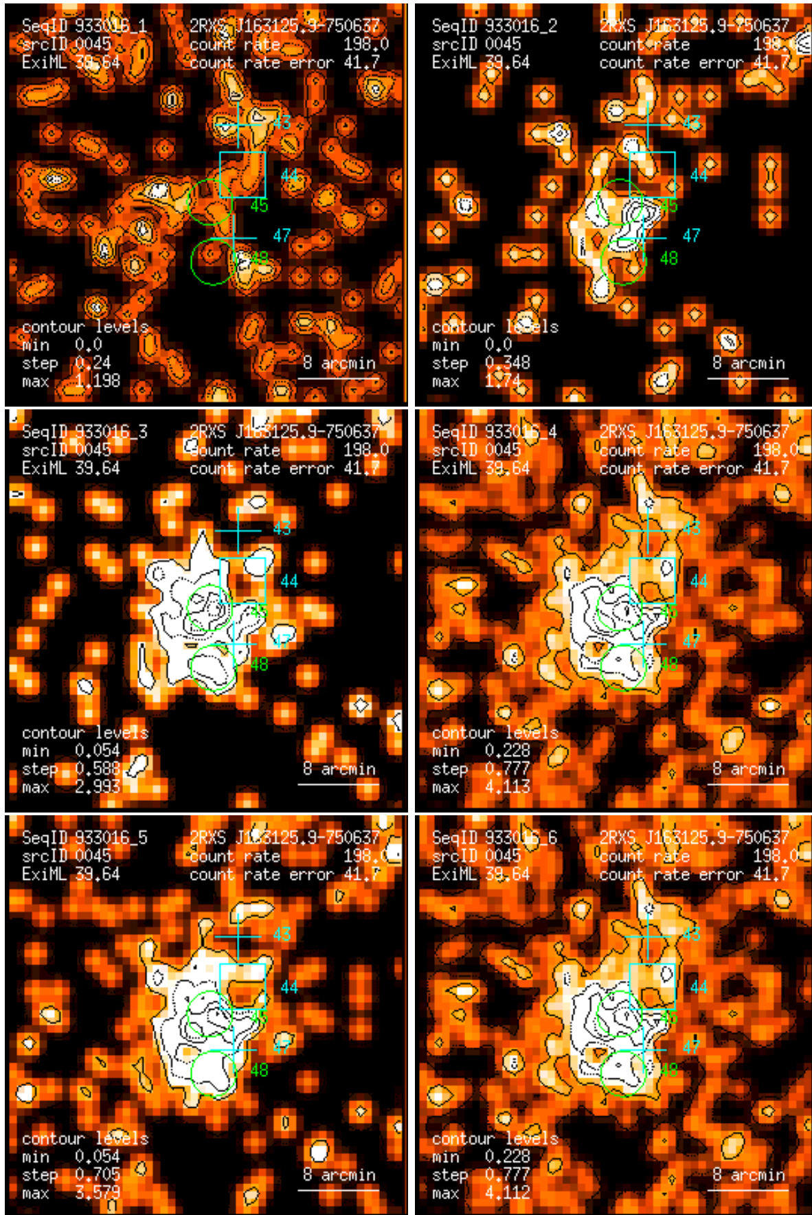
Figure 45: RASS 933016: detection 0045: band rate images, Gaussian filter: (1) PSPC channels 11 – 41, (2) 52 – 90, (3) 91 – 201, (4) 11 – 235, (5) 52 – 201, (6) 11 – 201. Broad band rates in counts/ks. Band rate contour levels in counts/ks/arcmin 2 .
