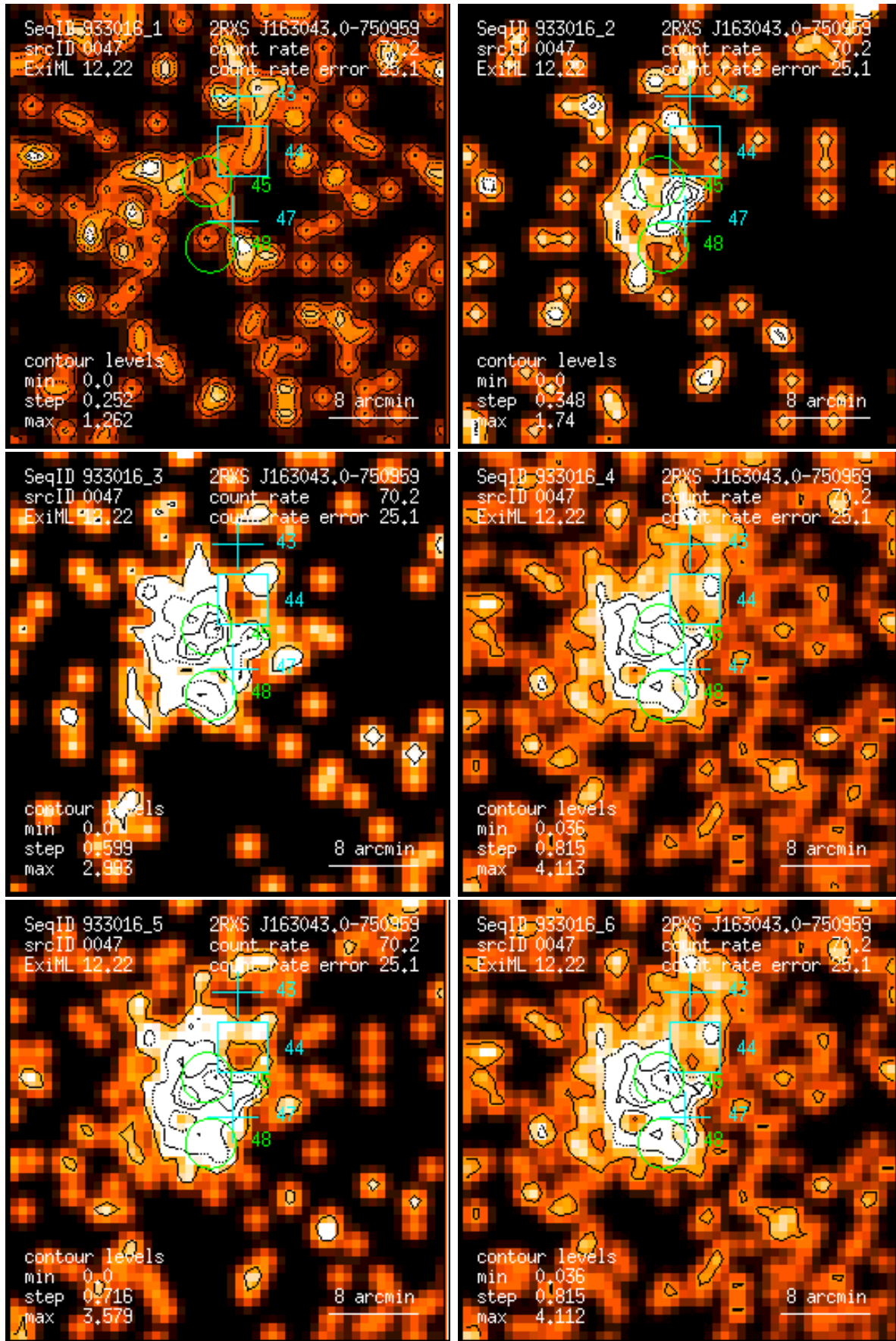
Figure 47: RASS 933016: detection 0047: band rate images, Gaussian filter: (1) PSPC channels 11 – 41, (2) 52 – 90, (3) 91 – 201, (4) 11 – 235, (5) 52 – 201, (6) 11 – 201. Broad band rates in counts/ks. Band rate contour levels in counts/ks/arcmin 2 .
