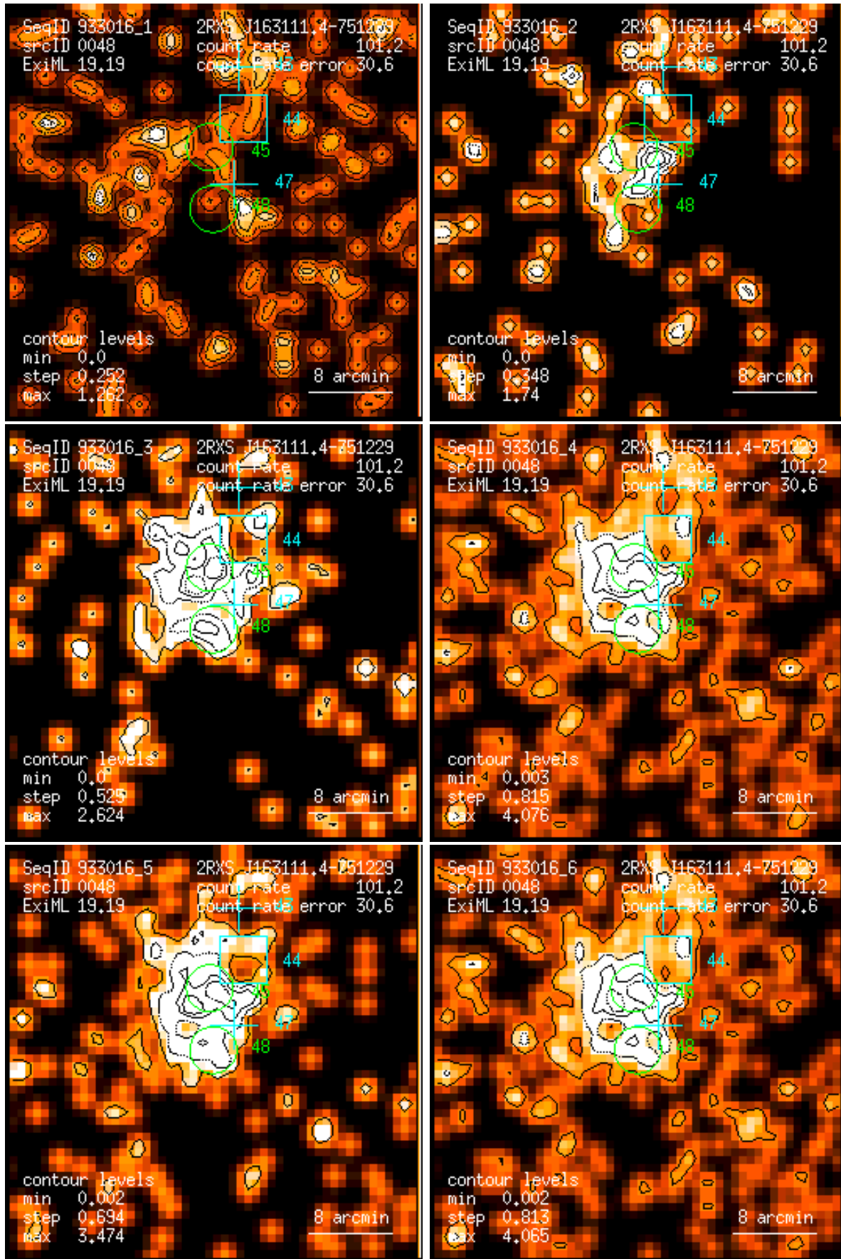
Figure 48: RASS 933016: detection 0048: band rate images, Gaussian filter: (1) PSPC channels 11 – 41, (2) 52 – 90, (3) 91 – 201, (4) 11 – 235, (5) 52 – 201, (6) 11 – 201. Broad band rates in counts/ks. Band rate contour levels in counts/ks/arcmin 2 .
