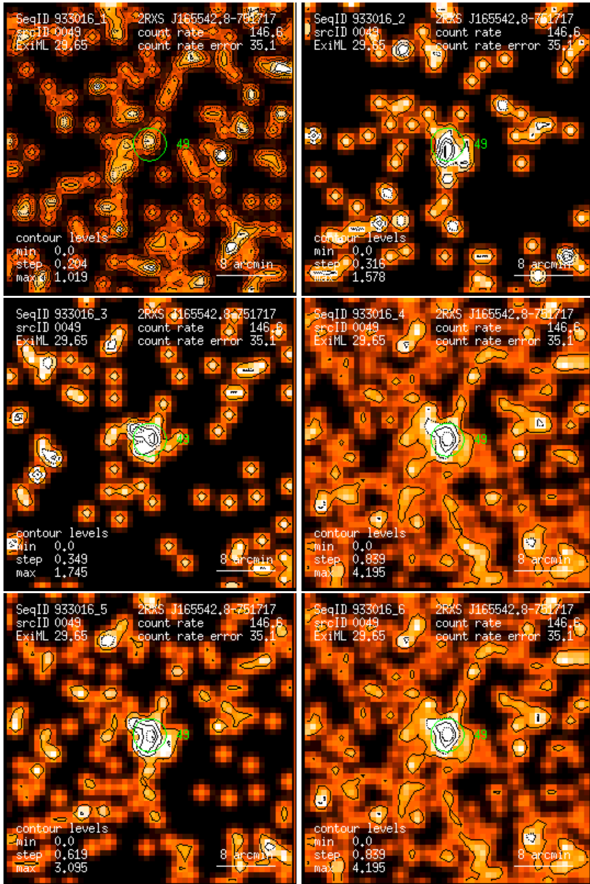
Figure 49: RASS 933016: detection 0049: band rate images, Gaussian filter: (1) PSPC channels 11 – 41, (2) 52 – 90, (3) 91 – 201, (4) 11 – 235, (5) 52 – 201, (6) 11 – 201. Broad band rates in counts/ks. Band rate contour levels in counts/ks/arcmin 2 .
