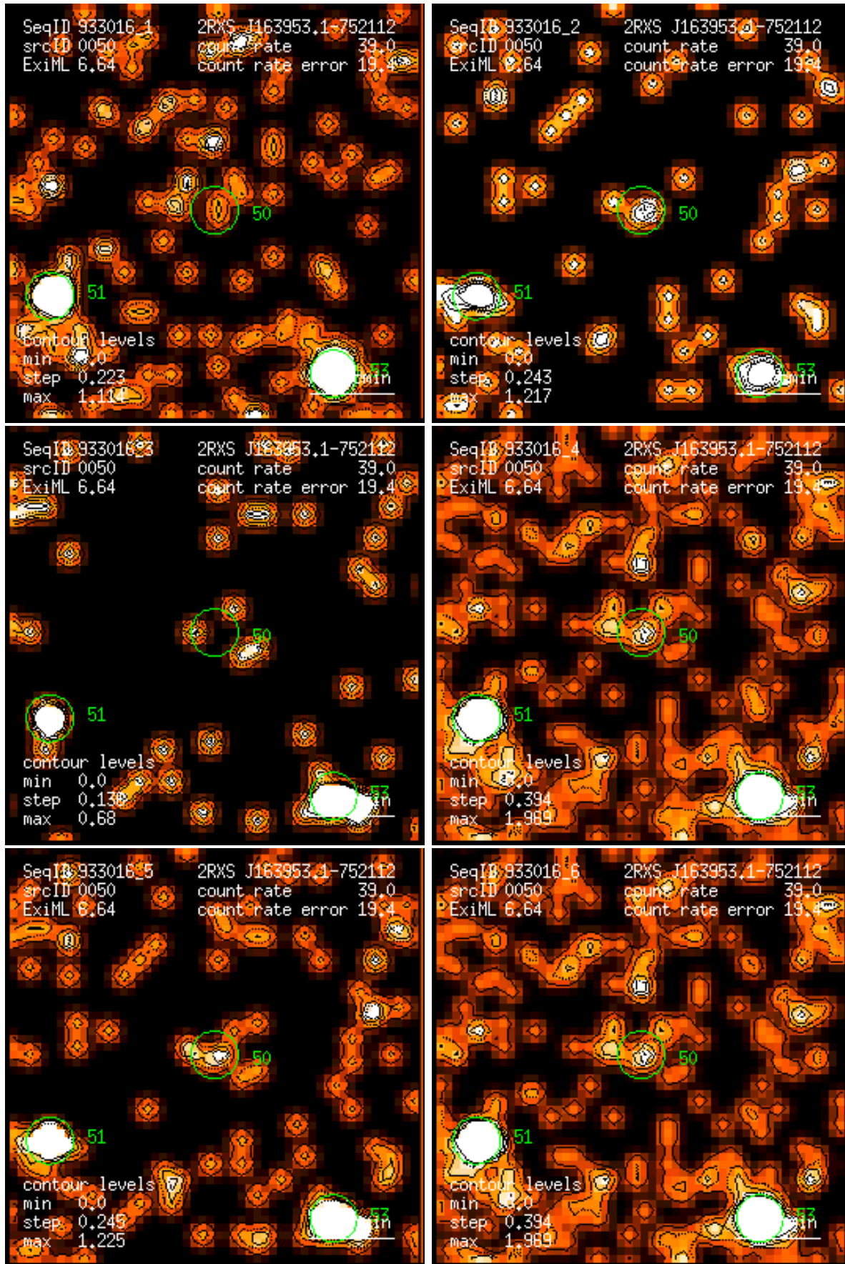
Figure 50: RASS 933016: detection 0050: band rate images, Gaussian filter: (1) PSPC channels 11 – 41, (2) 52 – 90, (3) 91 – 201, (4) 11 – 235, (5) 52 – 201, (6) 11 – 201. Broad band rates in counts/ks. Band rate contour levels in counts/ks/arcmin 2 .
