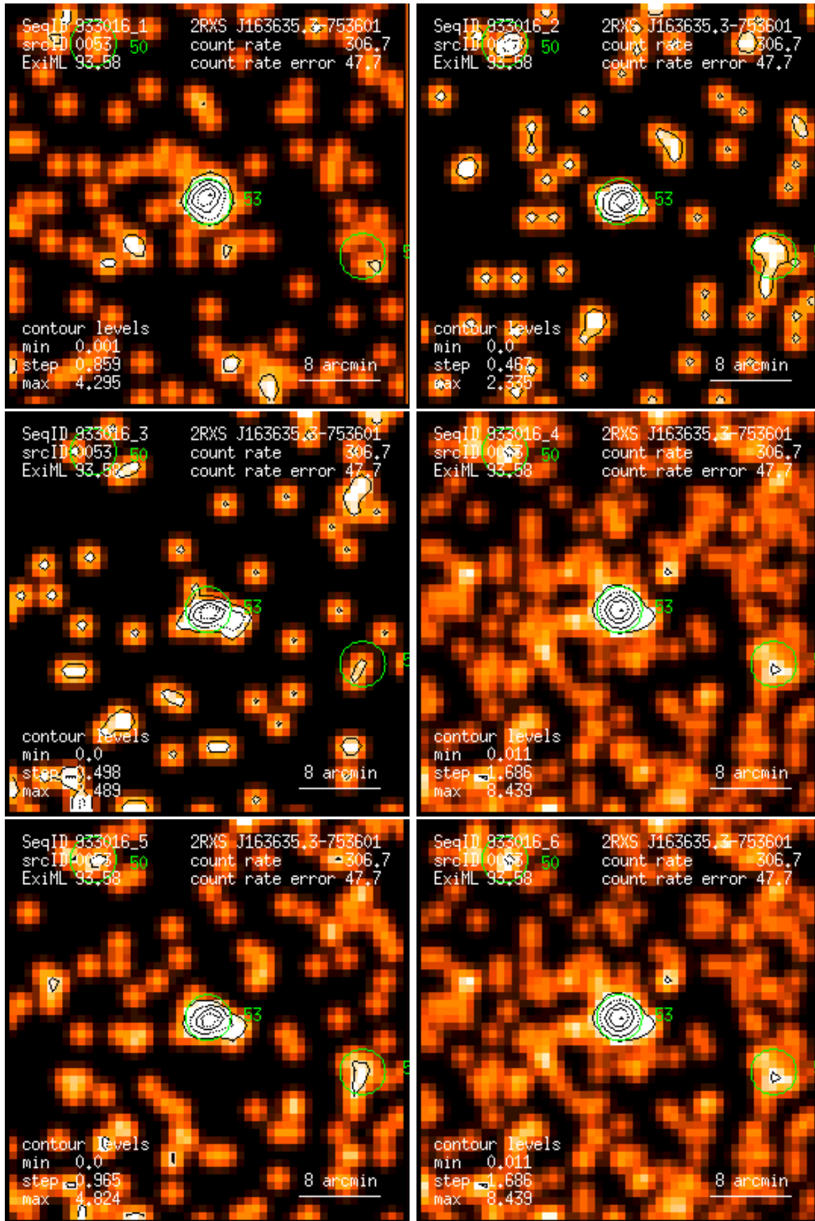
Figure 53: RASS 933016: detection 0053: band rate images, Gaussian filter: (1) PSPC channels 11 – 41, (2) 52 – 90, (3) 91 – 201, (4) 11 – 235, (5) 52 – 201, (6) 11 – 201. Broad band rates in counts/ks. Band rate contour levels in counts/ks/arcmin 2 .
